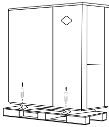
The heat pump is supplied mounted to a pallet. Once transported to site, remove the screws securing the pallet to the unit to install on the prepared slab / brackets.
