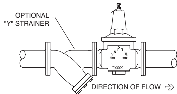
Horizontal Installation
