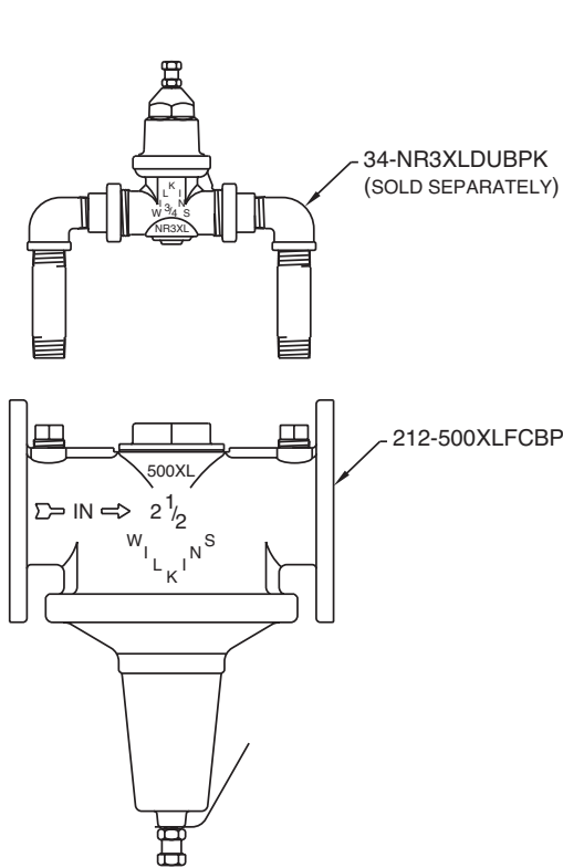
Parallel Installation
