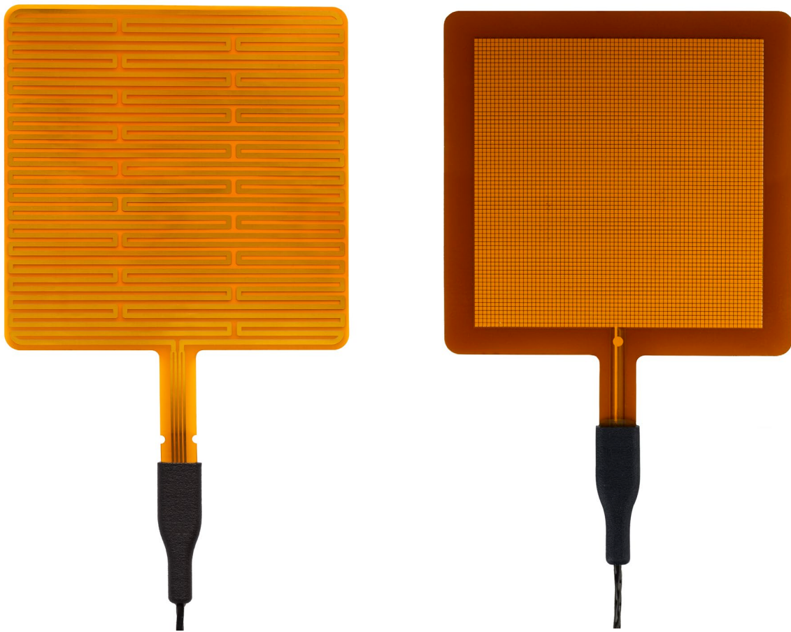
Figure 0.1 On the left: model HTR02-85X85 heater for calibration and verification of performance of the models of FHF05 series heat flux sensors. On the right: model HF05-85X85 to which HTR02-85X85 may be applied. See also Figure 3.2.1 for dimensions.
