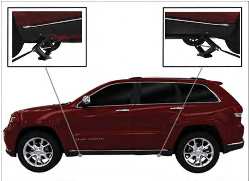
Jacking Locations
