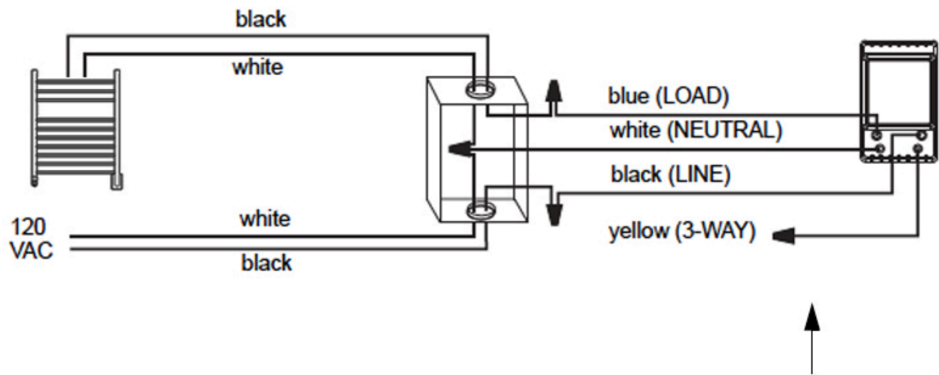
SINGLE-SWITCH INSTALLATION
