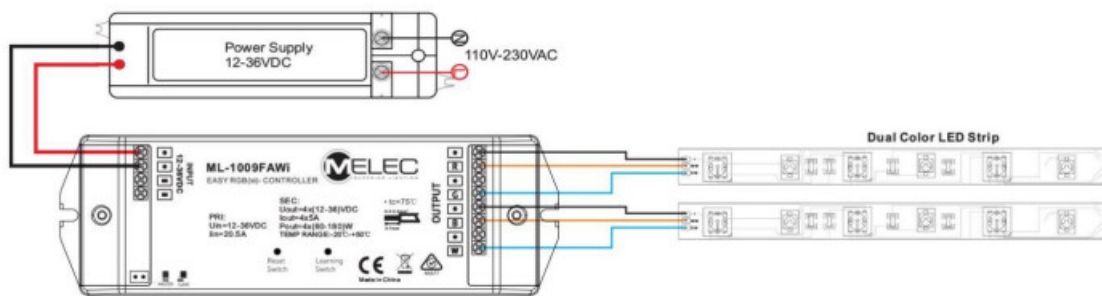
Dual Colour or Hybrid LED Strip
