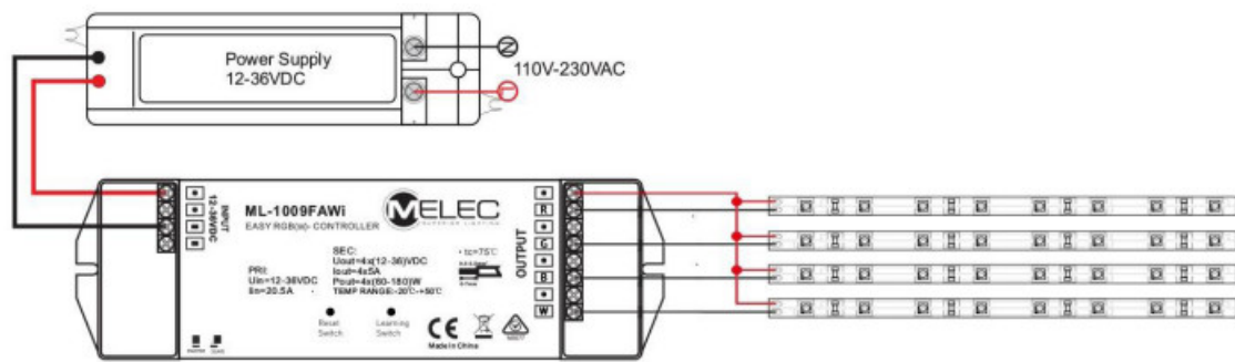
RGBW Connection Diagram
