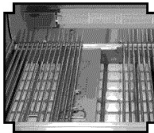
Figure 17-2 - Smoker box installed into grill for use.
