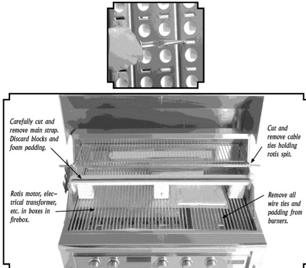
Figure 6-1 - Identification of items needing to be removed and/or assembled prior to use.
