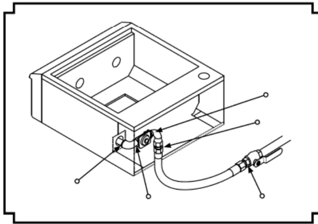
Figure II-1 - Leak testing points when using natural gas.
