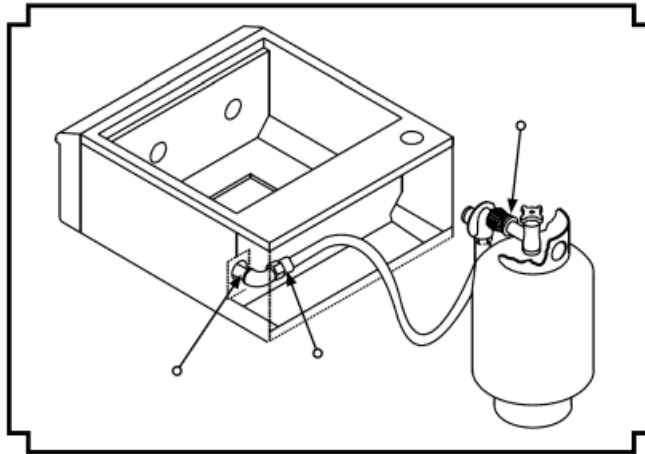
Figure II-2 - Leak testing points when using L.P. gas.
