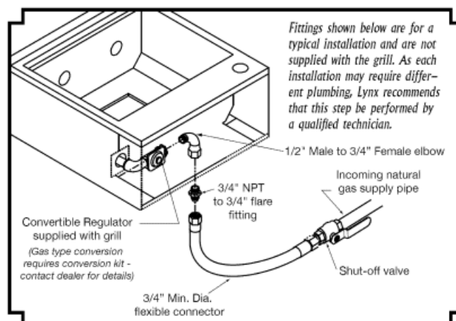
Figure 8-1 - Typical attachment for using natural gas.
