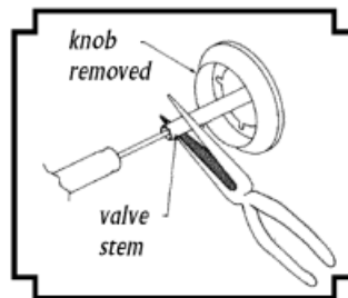
Figure 14-1 - Adjusting brass burner low heat setting.
