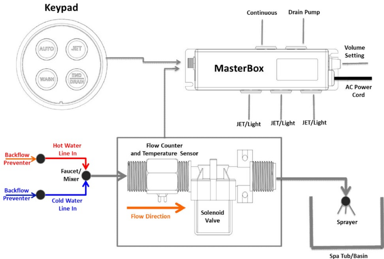
Fig.1: Connection Diagram
