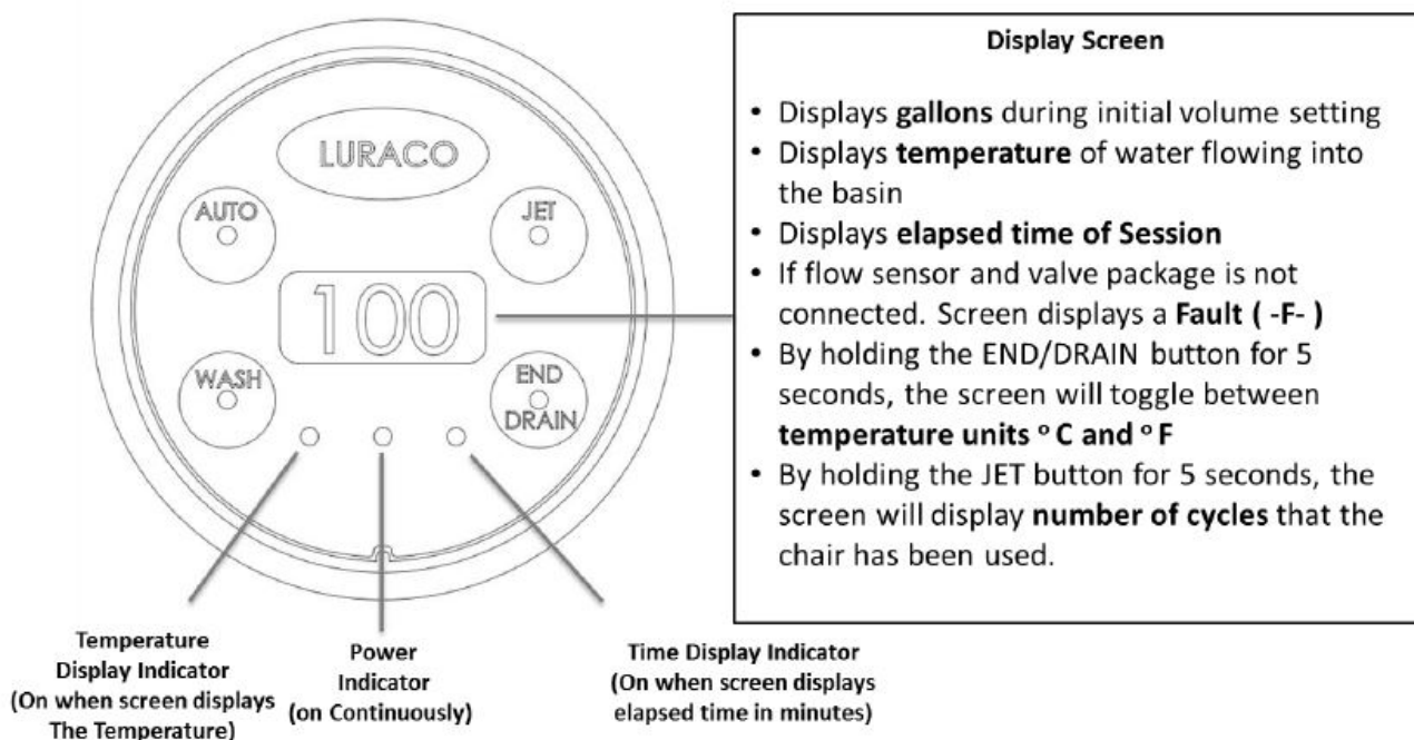
Fig.2: Display Screen
