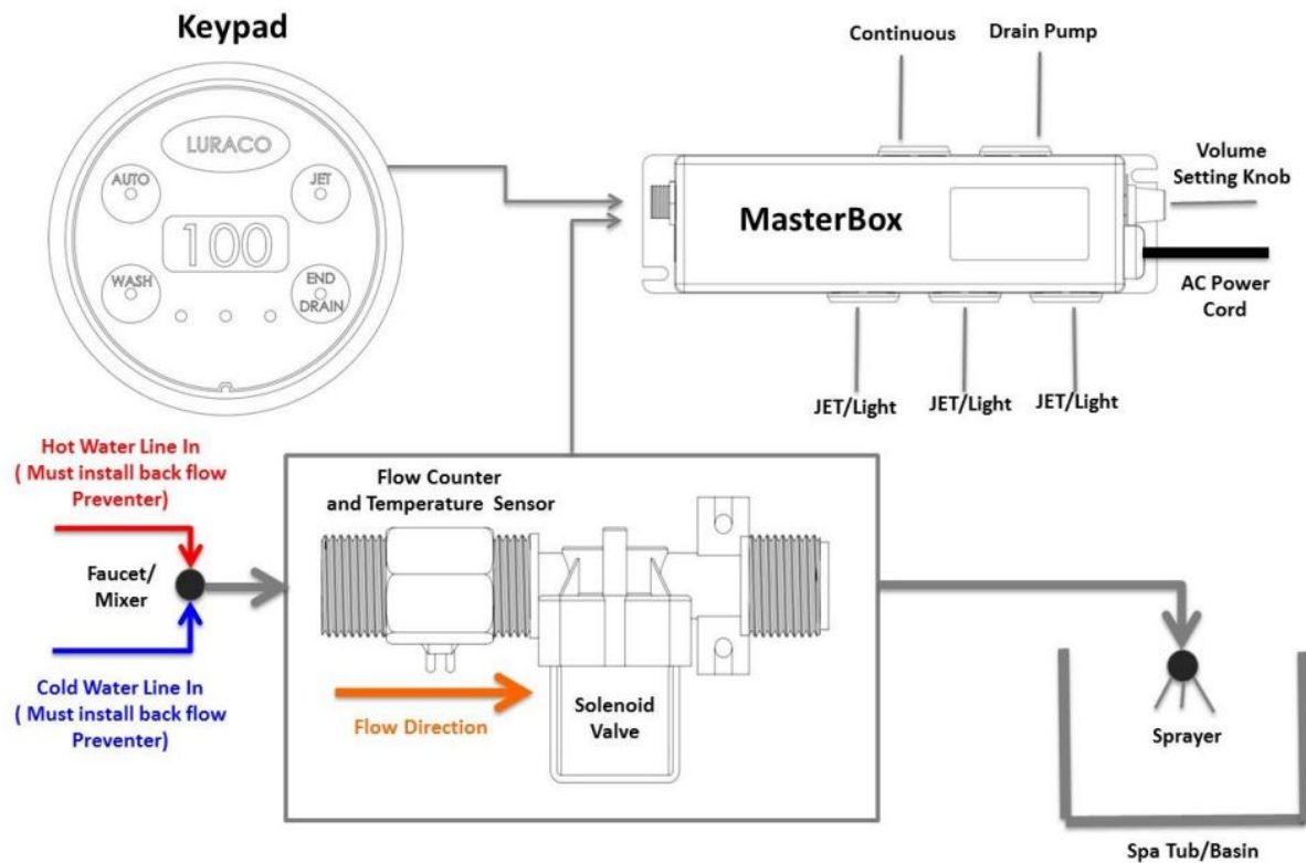
Fig.1: Connection Diagram
