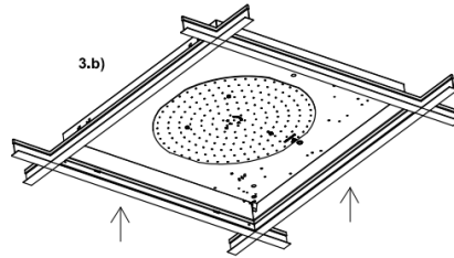
GB - Install geartray (if ELFIX luminaire). Remember to connect Internal plug connection.
