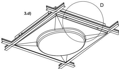
GB - Gently push beneath the tabs with your fingers so, that the tabs are pushed into the luminaire box and then push the opalcover up into place in the luminaire.
