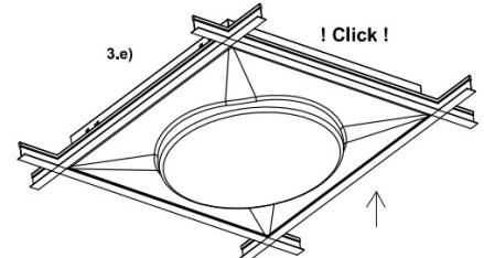
GB - When the opalcover is "clicked" safely into place, the installation is done.
