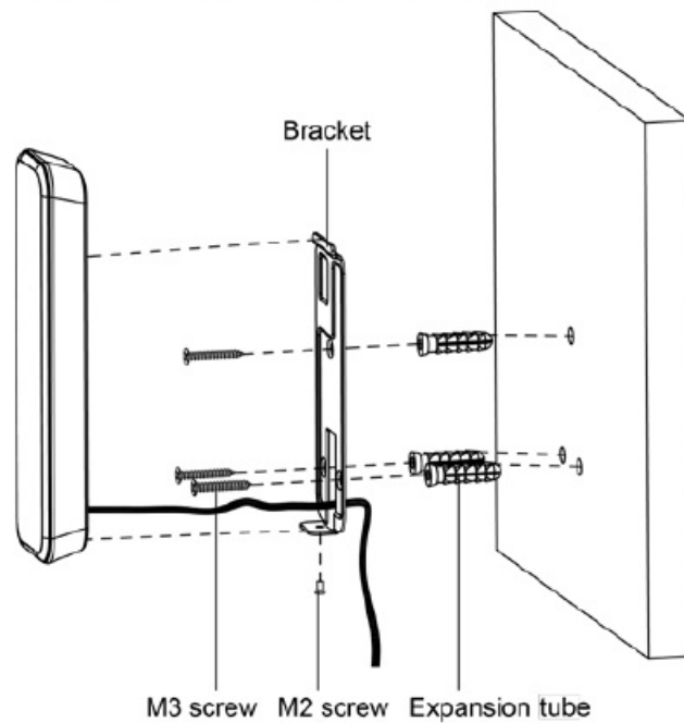
Figure 3-2 Surface mounted wiring
