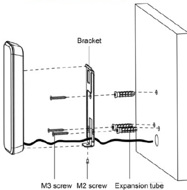
Figure 3-1 In-wall wiring
