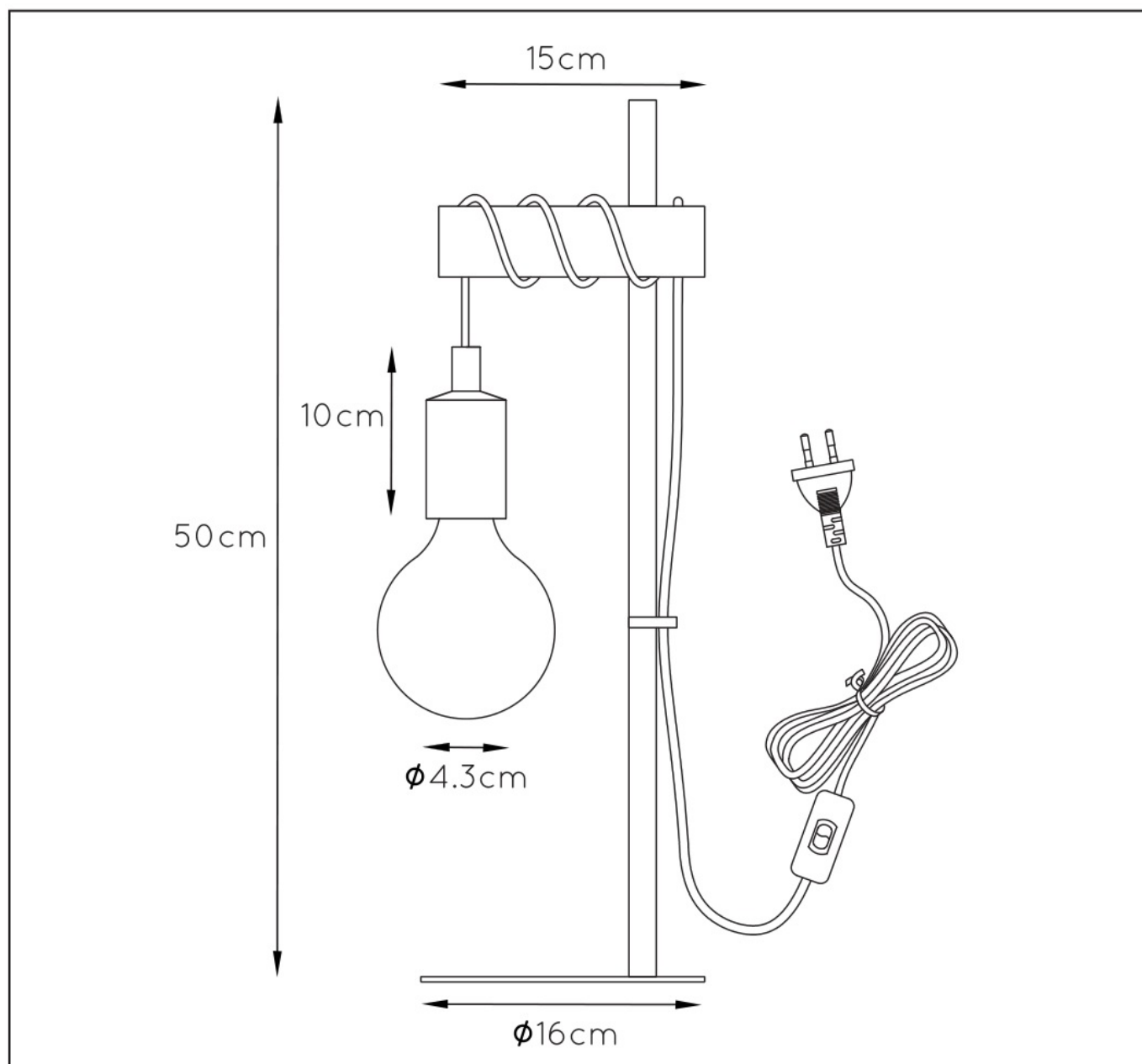
INSTALLATION DRAWING SPECIFICATIONS
