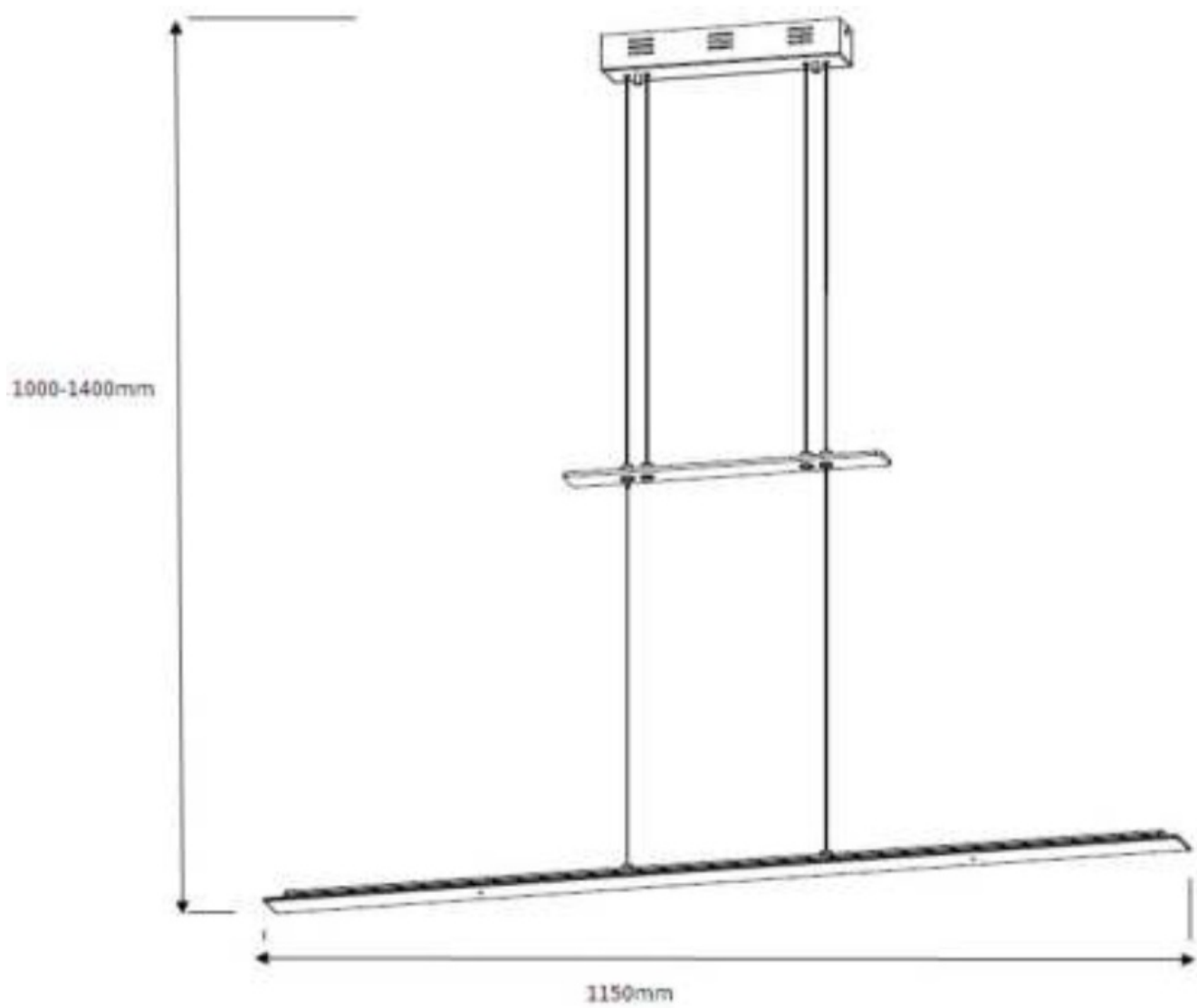
Installation drawing
