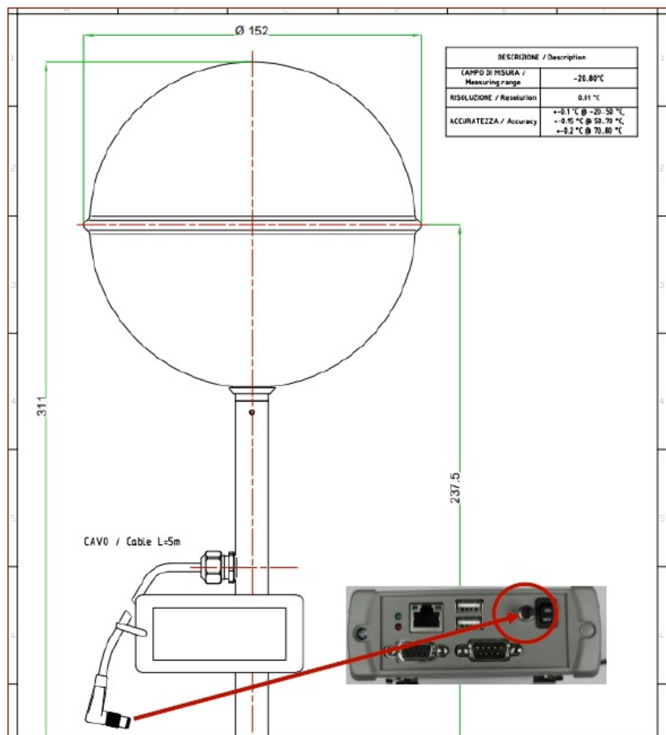
PRTEA4922.1 sensor schematic drawing
