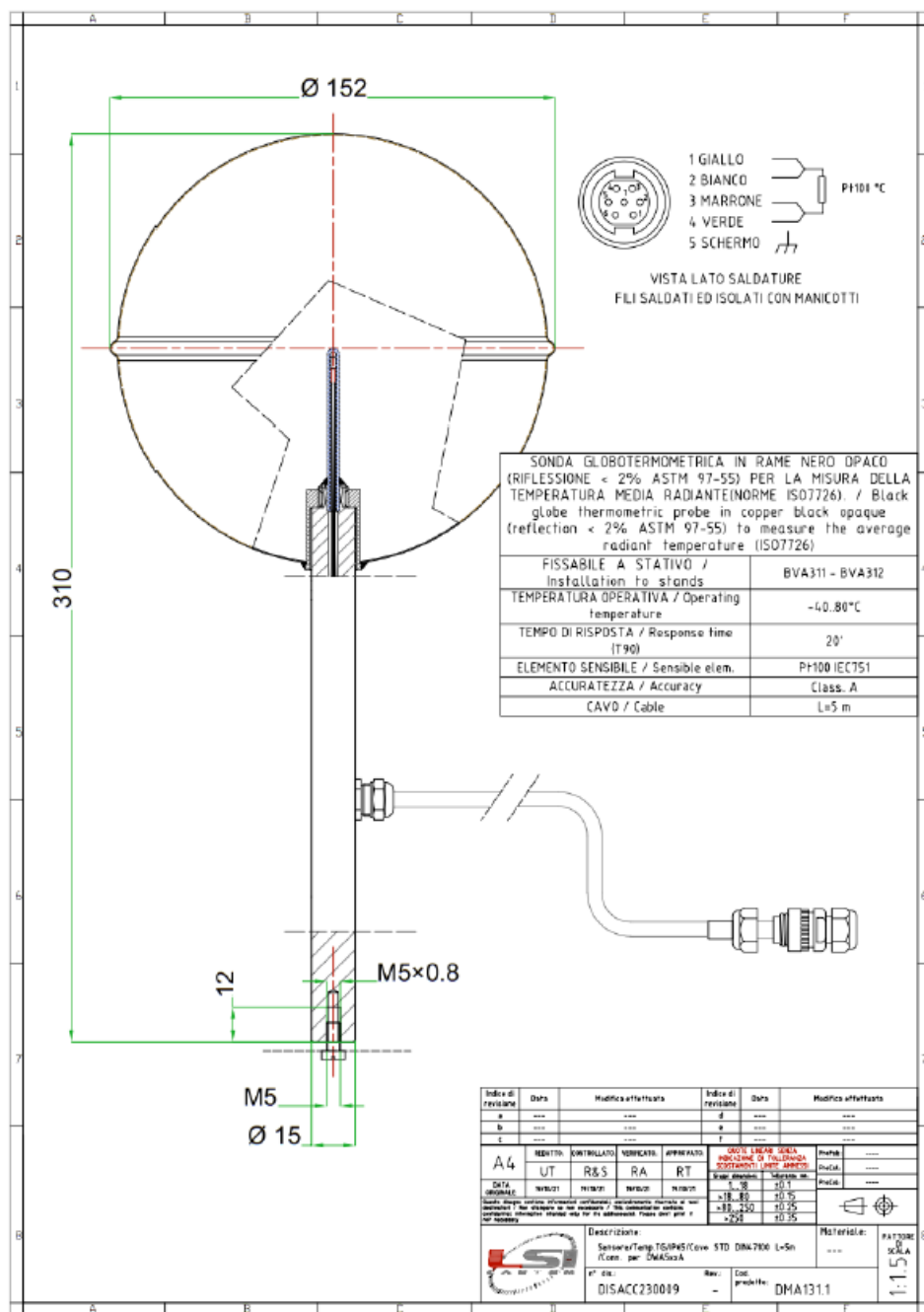
PRTEA4922 sensor schematic drawing to Alpha-Log data logger
