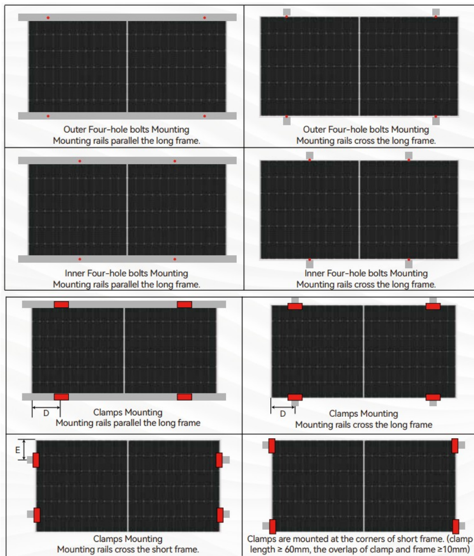
Figure 8 Bifacial Module Installation Position
