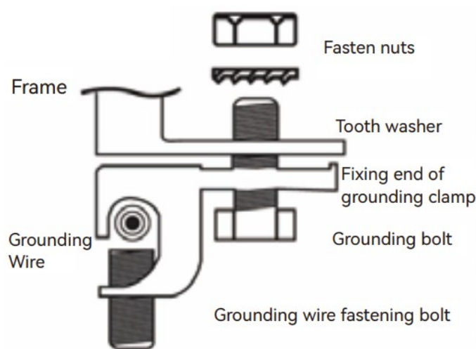
Figure 10 Bolt Grounding Method of PV Module
