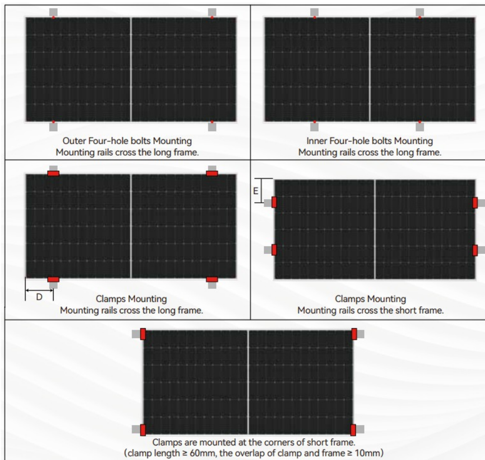
Figure 7 Mono-facial Module Installation Position
