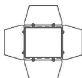
Four-way Barndoor × 2
