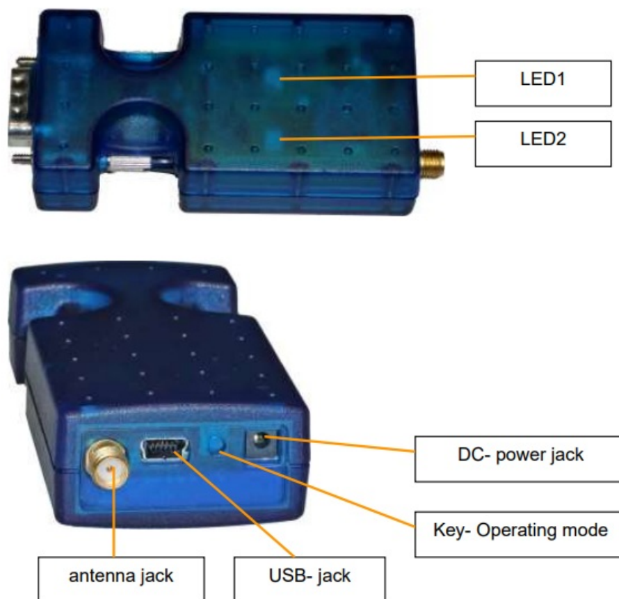
Illustration 1 View of Bluetooth RS232 Mini Adapter/S
