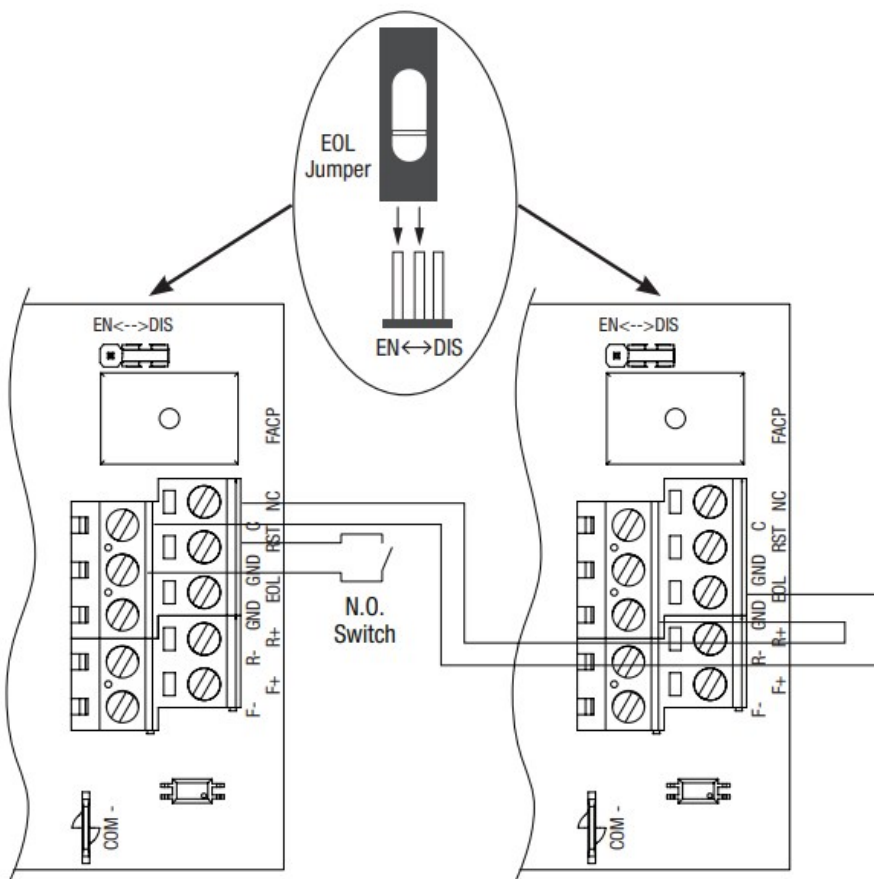
Fig. 8 – Daisy chaining one or more LINQ8ACM(CB) units. EOL Jumper [EOL JMP] (Fig. 5, pg. 5, Z) should be installed in the “EN” position. Latching Individual Reset.
