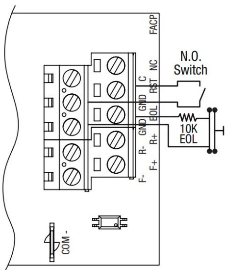
Fig. 13 – Normally Open trigger input (Non-Latching).
