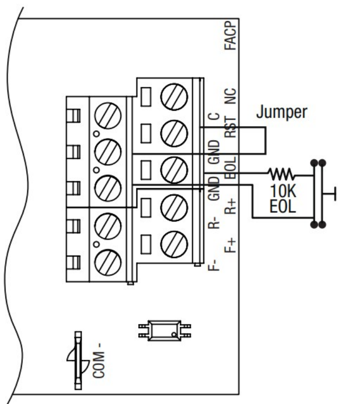
Fig. 12 – Normally Closed trigger input (Latching).
