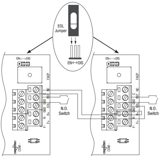
Fig. 9 – Polarity reversal input from FACP signaling circuit output (polarity is referenced in alarm condition). Non-Latching.
