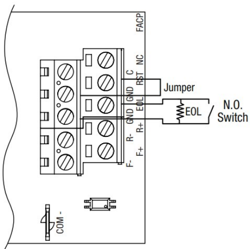
Fig. 14 – Normally Open trigger input (Latching).
