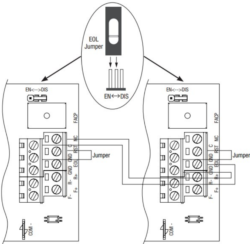
Fig. 7 – Daisy-chaining one or more LINQ8ACM(CB) units. EOL Jumper [EOL JMP] (Fig. 5, pg. 5, Z) should be installed in the “EN” position. Latching Single Reset.
