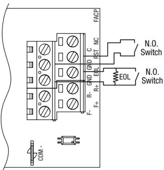
Fig. 14 – Normally Open trigger input (Latching).
