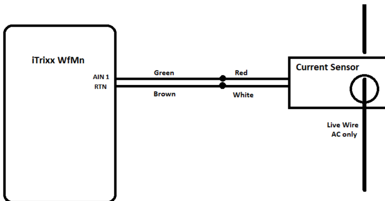
Current Sensor Wiring Diagram
