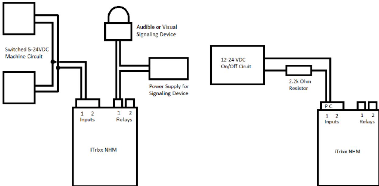
Left: iTrixx NHM wiring; Relay Output Connection circuit to digital input using 2.2k ohm inline resistor
