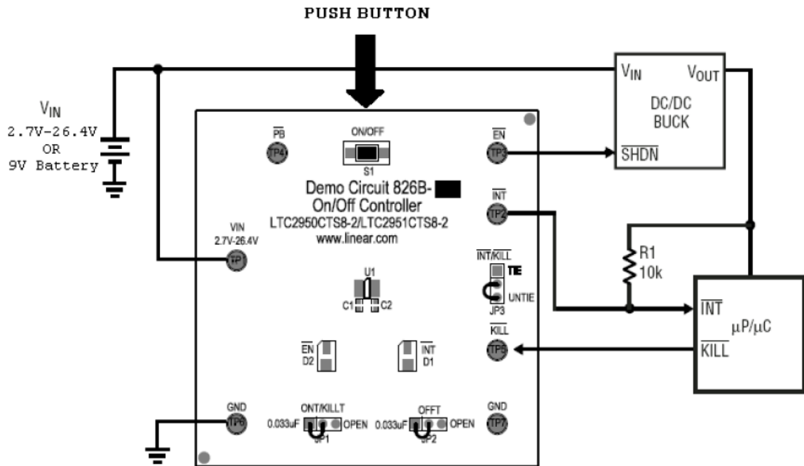
Figure 1. DC826B-A/DC826B-B Example Setup
