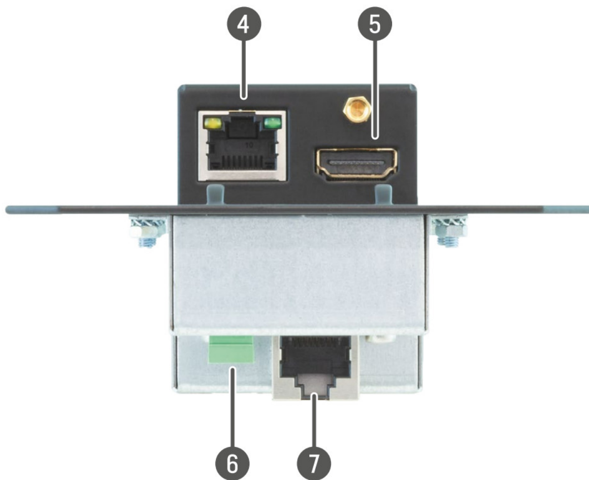
Bottom View (WP-HDMI-TPS-RX97-FP-8AT model)
