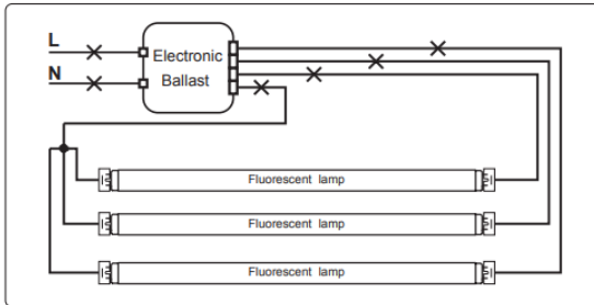
Retrofit luminaire with 3 lamps
