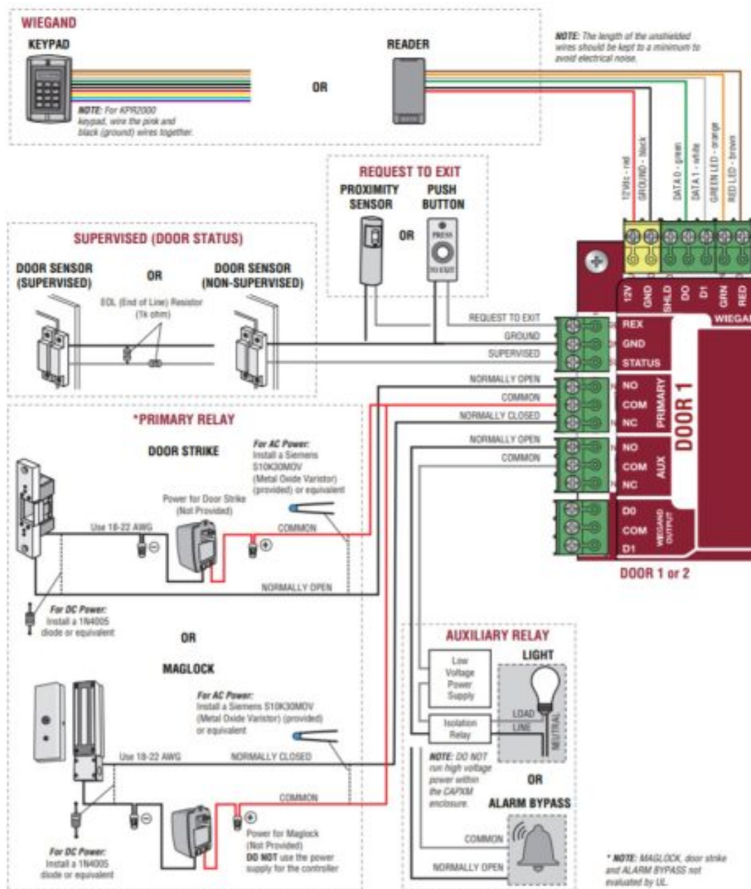
LiftMaster LMSC1000 RFID Reader Wiring Diagram
