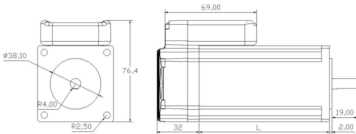
1/ Motor installation dimension drawing
