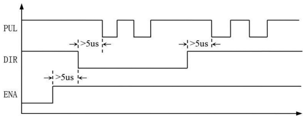
5/ Control signal timing diagram
