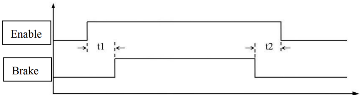
6/ Motor brake signal control timing diagram
