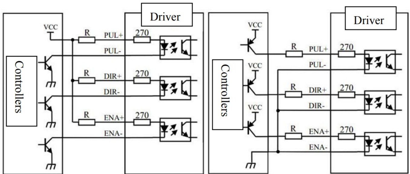
2/ Common anode connection
