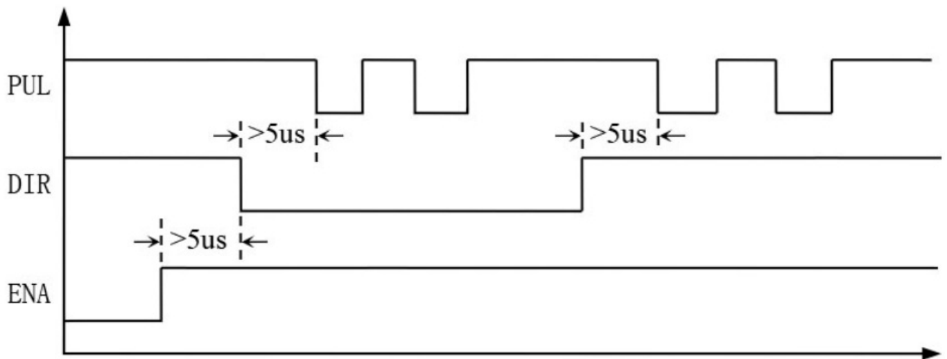
Figure 5 Control signal sequence diagram
