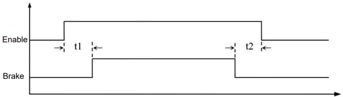
Figure 6 Motor brake control signal timing diagram
