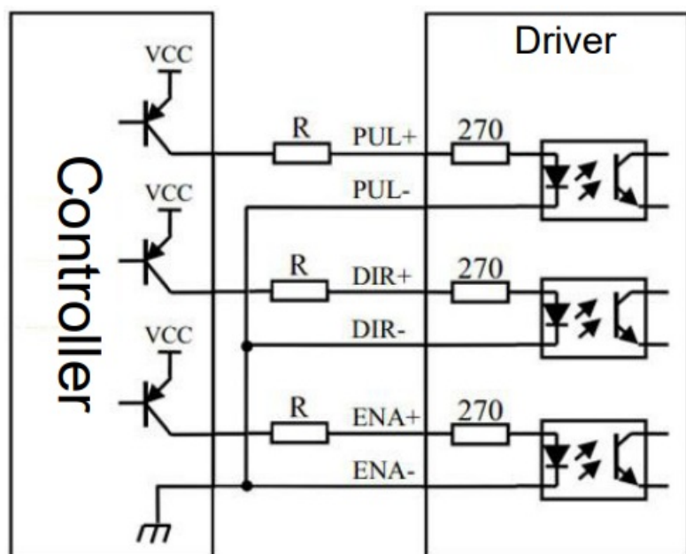
Figure 3 Common cathode connection
