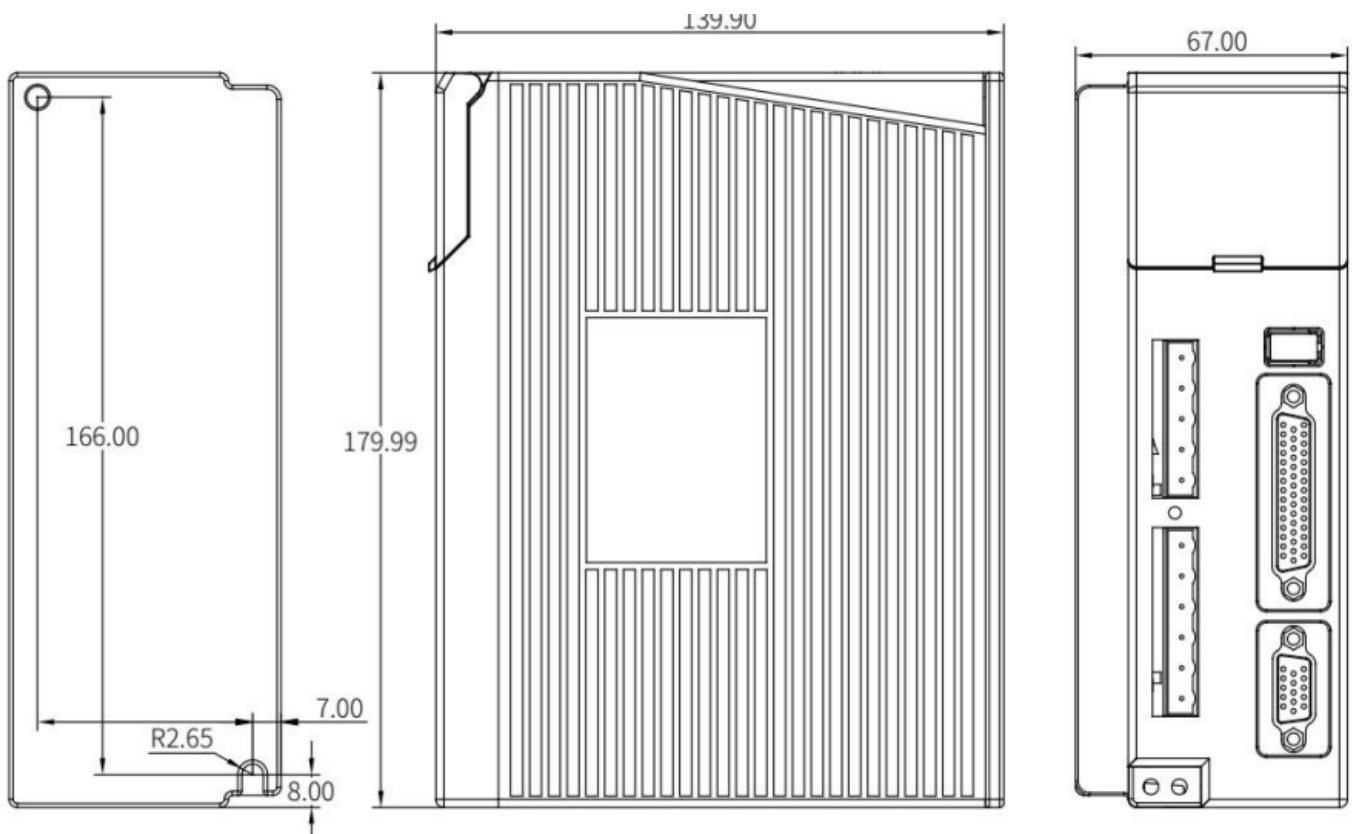
Figure 1 Drive mounting dimensions drawing
