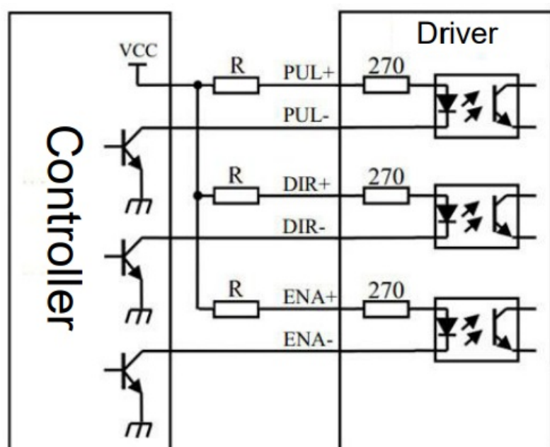
Figure 2 Common anode connection
