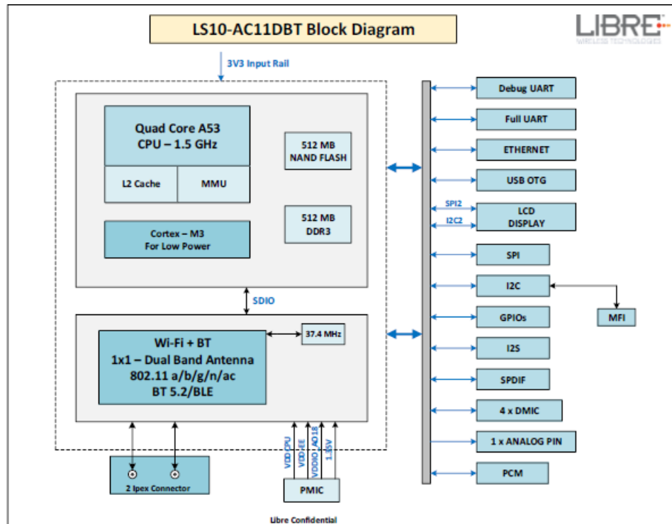
Figure 5-1: LS10 MODULE Block Diagram
