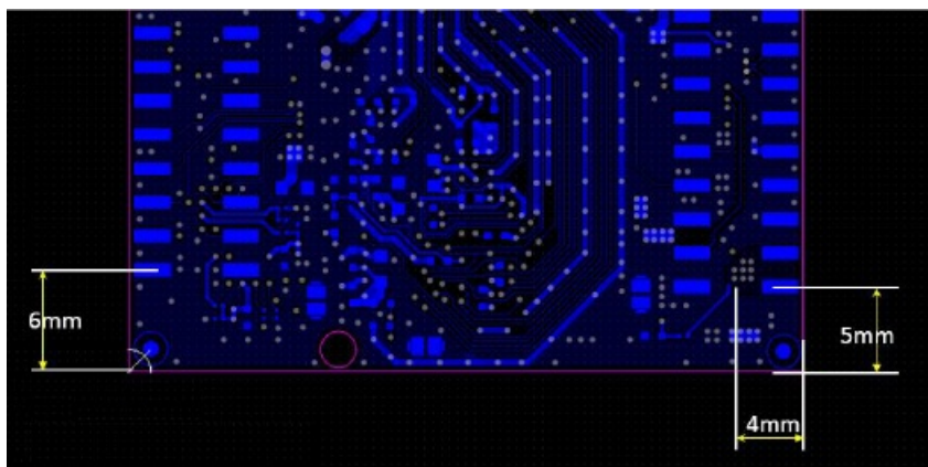
7.1-4: LS10 Top View – Mechanical Dimension 2
