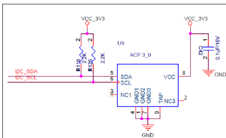
Figure 9.2-1: LS10 EVK ACP 3.0
