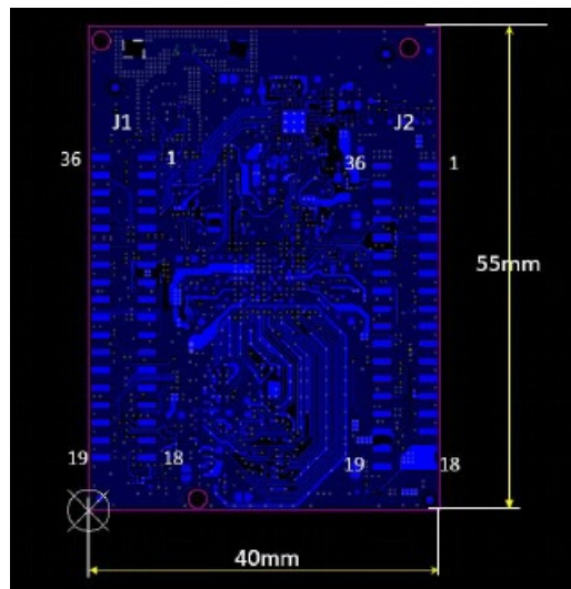
Figure 7.1-3: LS10 Top View – Mechanical Dimension 1
