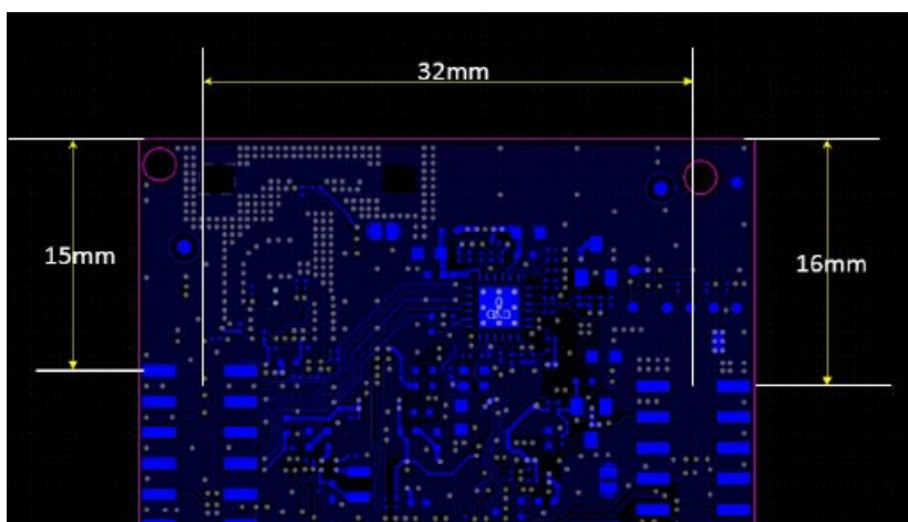
Figure 7.1-5: LS10 Top View – Mechanical Dimension 3
