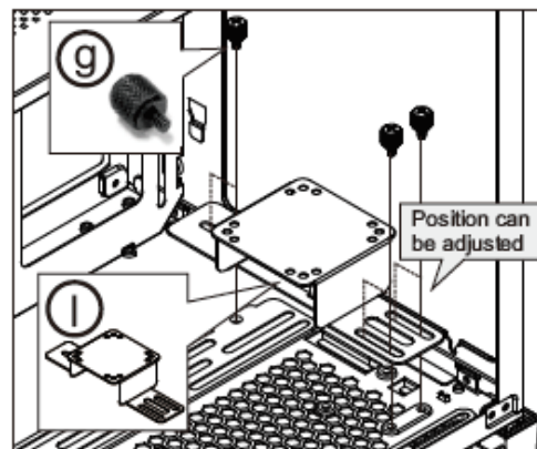
Water pump bracket 2 installation
