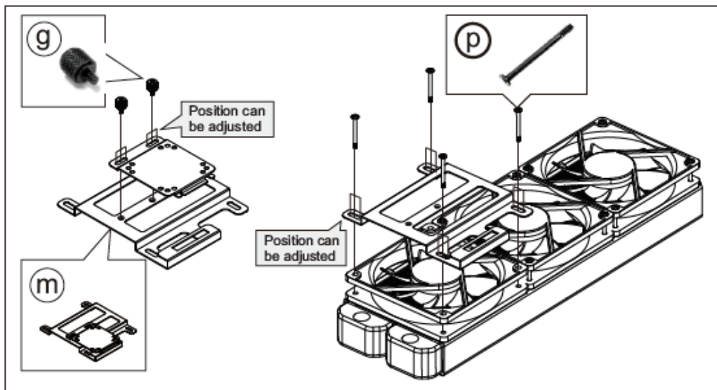
Water pump bracket 3 installation
