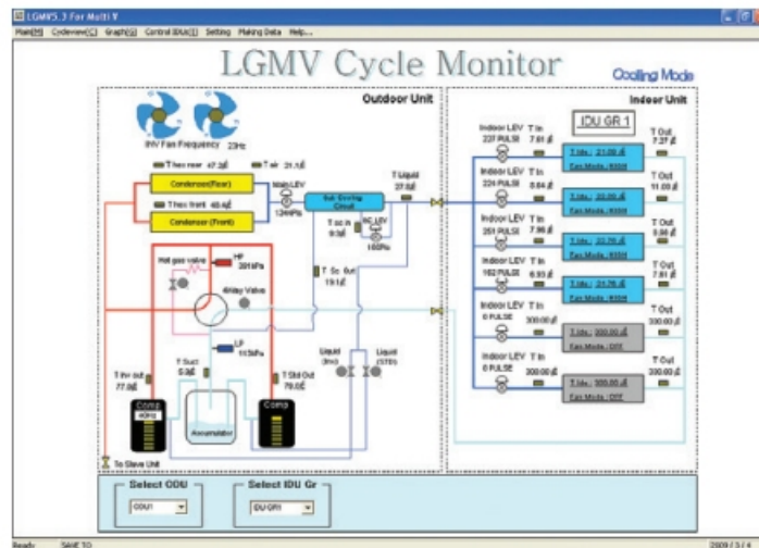
Figure 45: Sample Cycleview.
