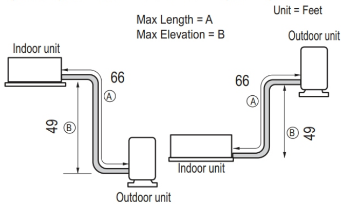
Figure 59: Typical LC098HV4 and LC128HV4 System Layout.
