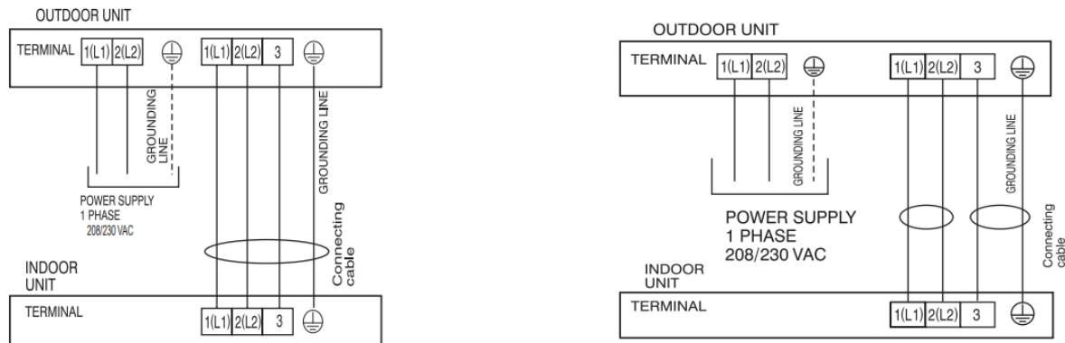
Figure 34: Schematic of a Single Zone Cassette System When the Wiring is GREATER THAN 130 Feet.
