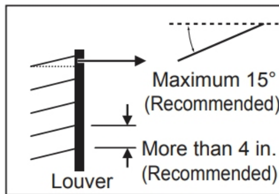
Figure 55: Louver Recommendations.
