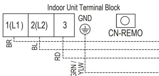
Figure 37: Wired Controller Connection (Example Only).
