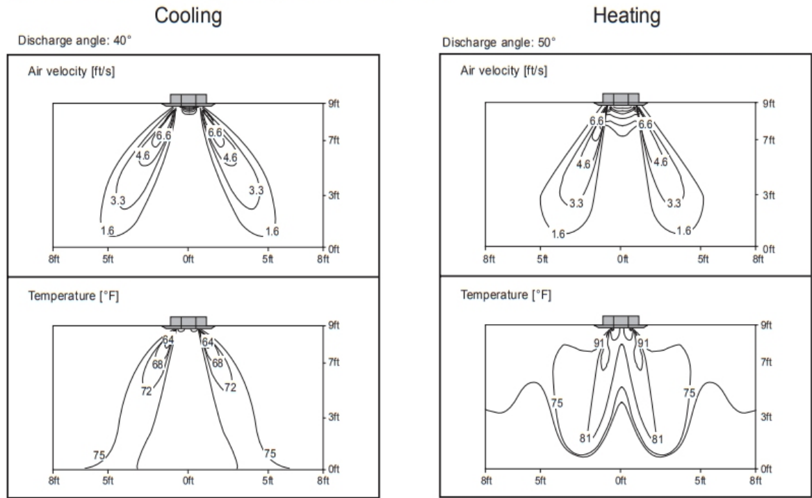
Figure 40: LCN128HV4 Air Velocity and Temperature Distribution Charts.
