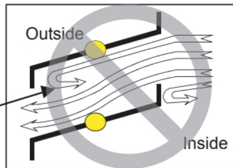
Figure 56: Using "S" Type Louvers.
