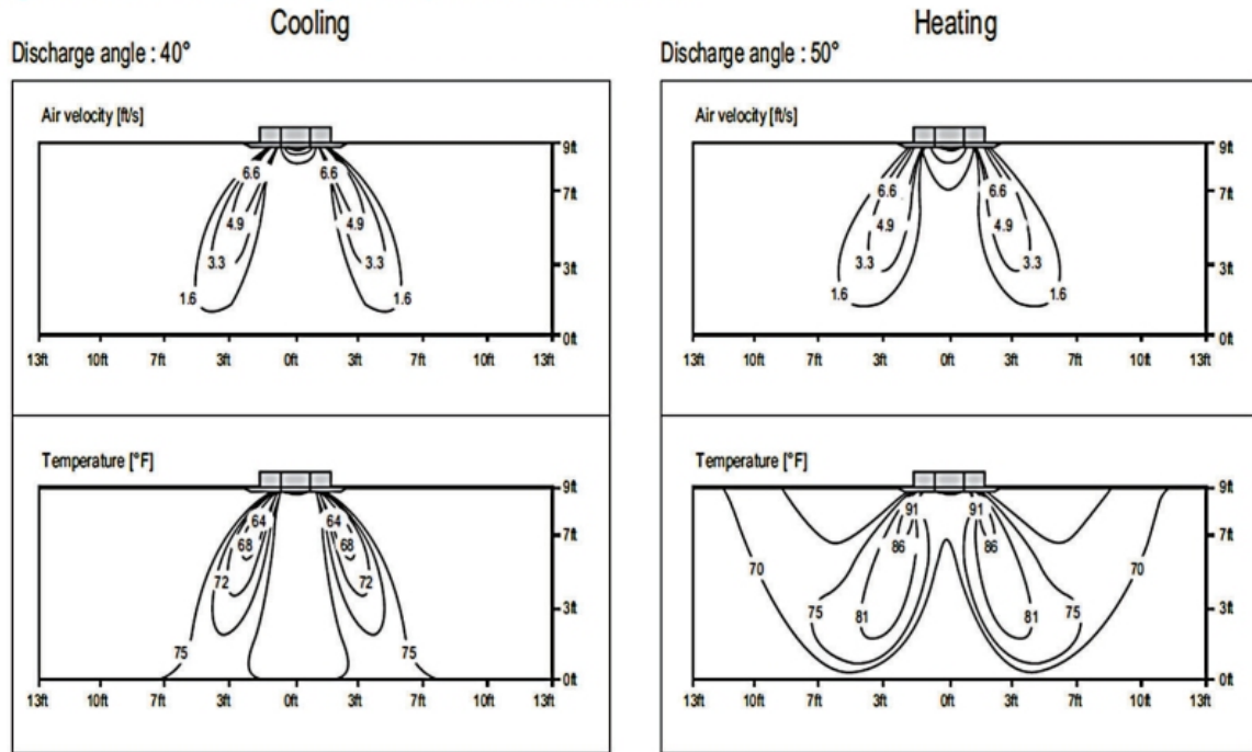
Figure 41: LCN188HV4 Air Velocity and Temperature Distribution Charts.
