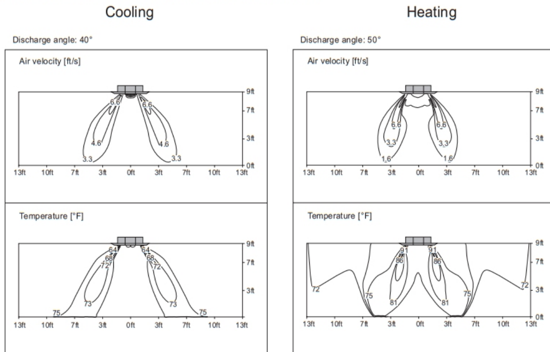
Figure 42: LCN248HV Air Velocity and Temperature Distribution Charts.
