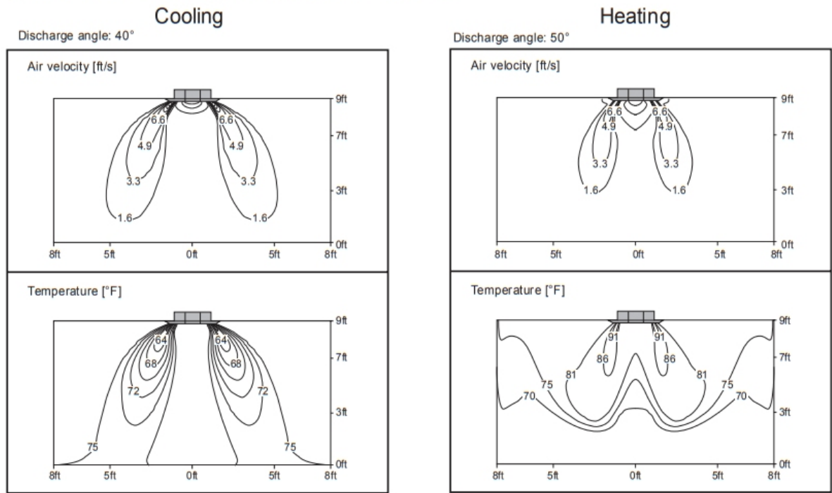
Figure 39: LCN098HV4 Air Velocity and Temperature Distribution Charts.
