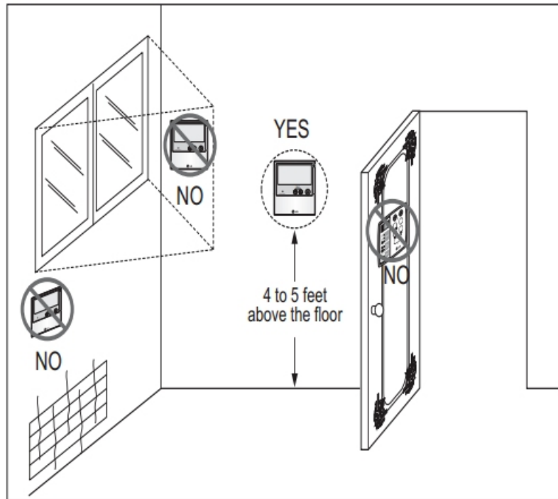
Figure 38: Proper Location for the Wired Controller
