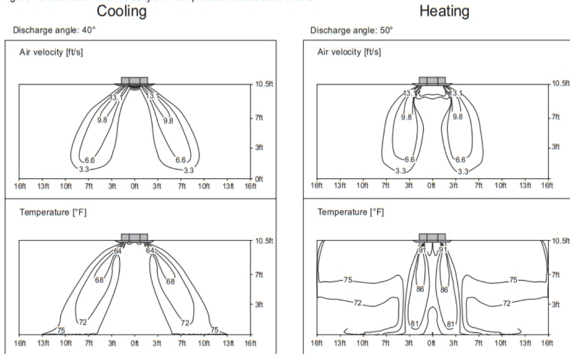
Figure 44: LCN428HV Air Velocity and Temperature Distribution Charts.
