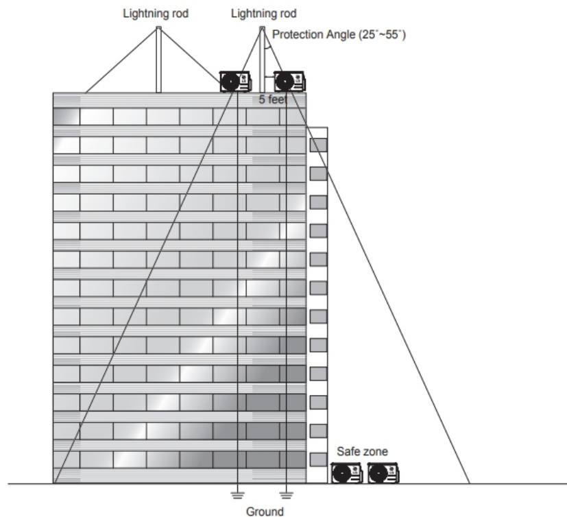
Figure 51: Lightning Protection Diagram.
