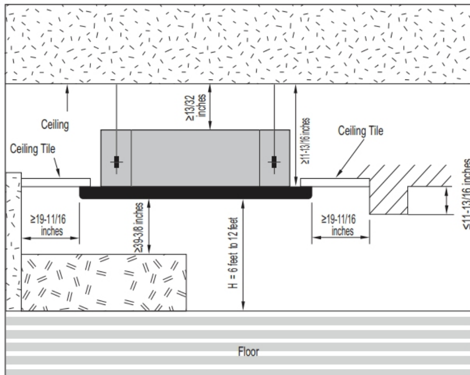
Figure 47: Indoor Unit Clearance Requirements.
