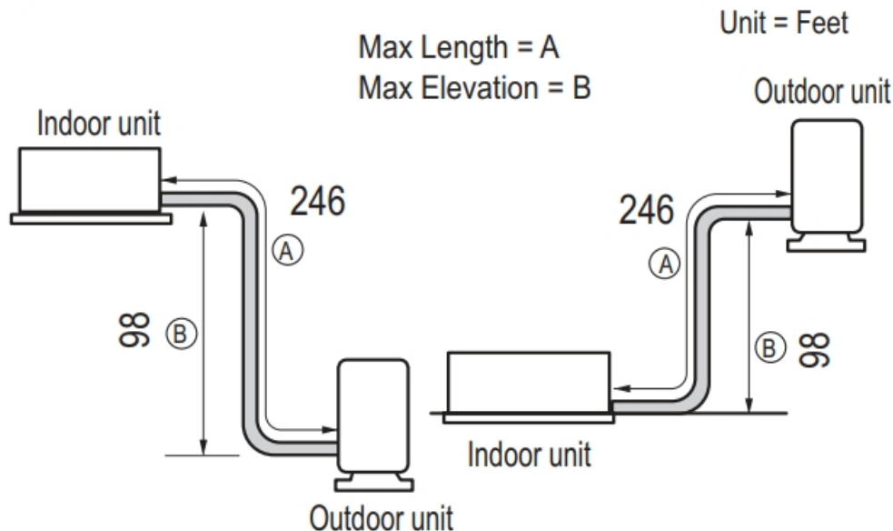
Figure 61: Typical LC348HV4 and LC428HV System Layout.
