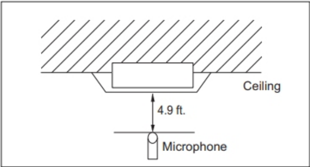
Figure 12: Indoor Unit Sound Pressure Level Measurement Location.
