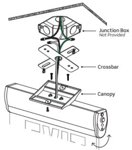
Ceiling Mount
