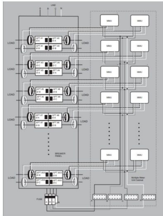
Three-Phase, 4-Wire Hookup Diagram
