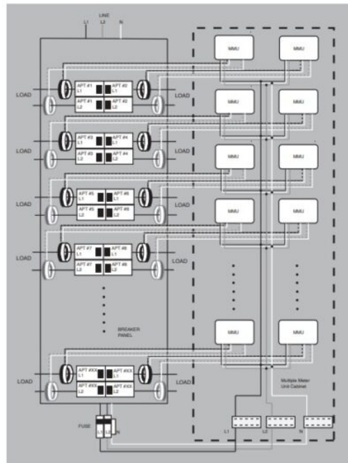
Two-Phase (Split Phase), 3-Wire Hookup Diagram
