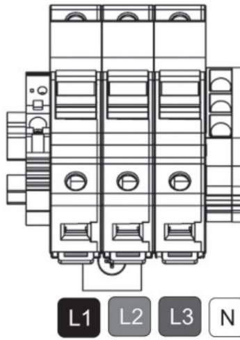
Voltage Terminal Block Connections
