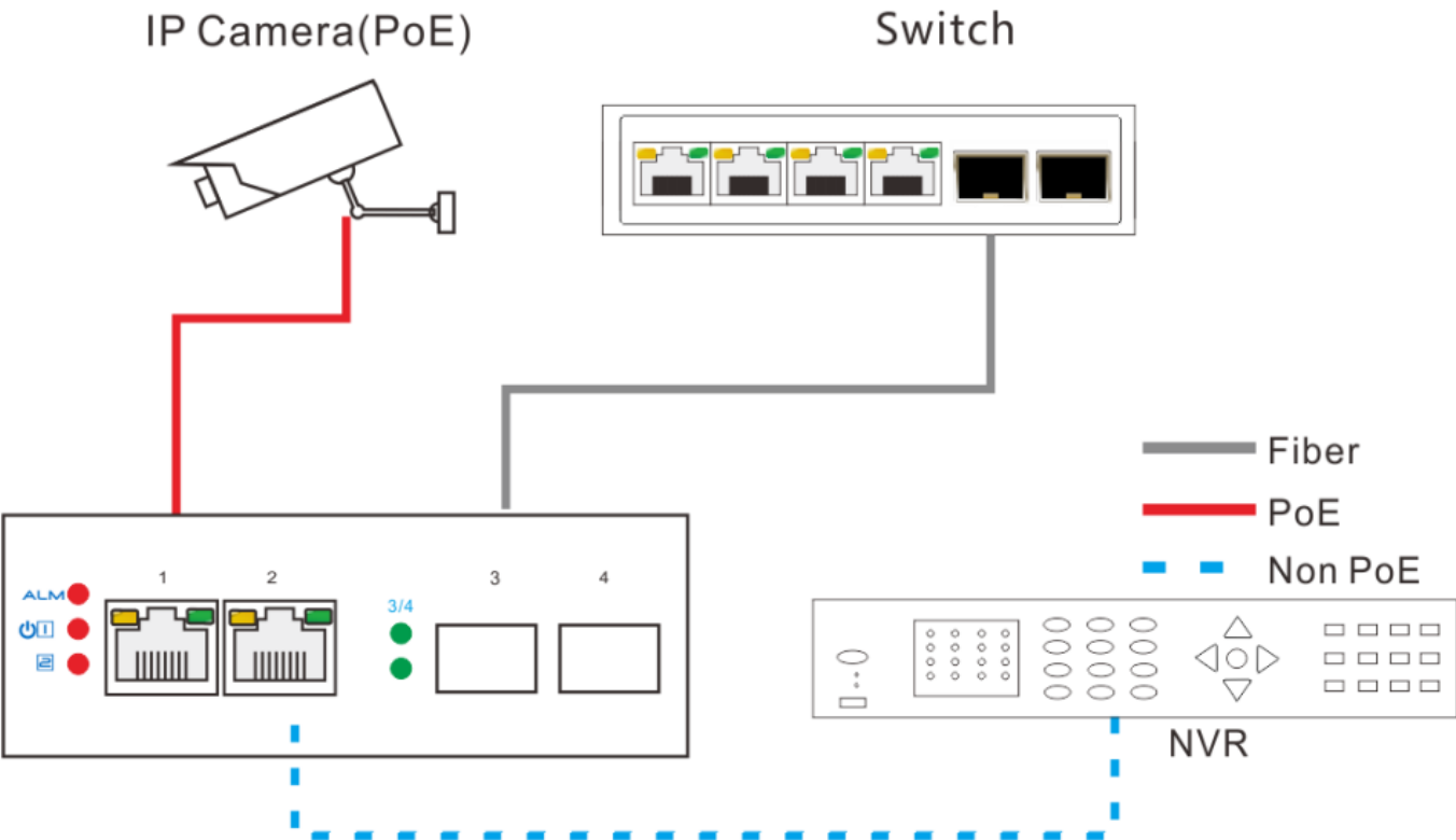
Installation diagram
