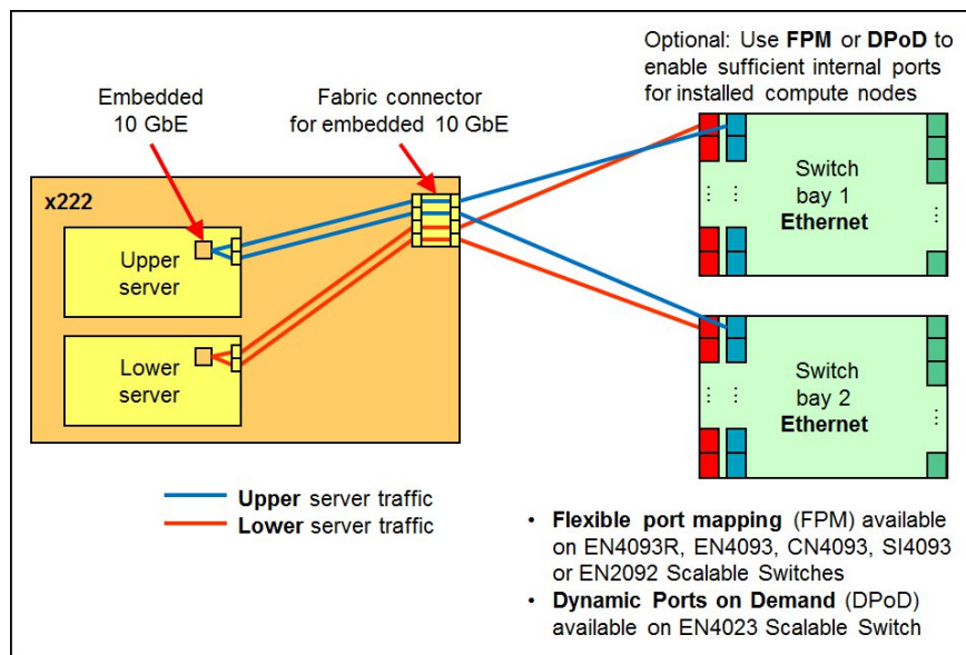
Figure 6. Embedded two-port 10 Gb VFA connectivity to the switches In the figure:
