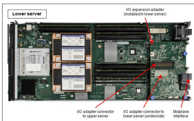
Figure 7. Location of the I/O adapter
