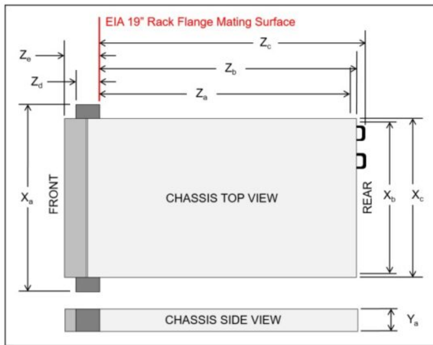
Figure 21. Server dimensions
