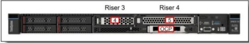
Figure 12. SR635 V3 front slots
