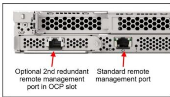
Figure 19. SR635 V3 with the Redundant System Management Port Adapter installed
