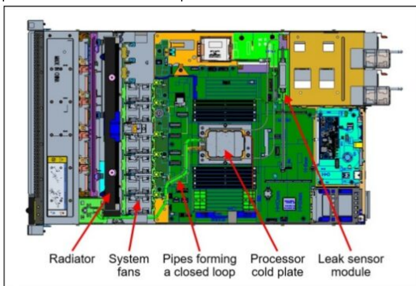
Figure 6. SR635 V3 with closed loop heatsink (feature BS34)
