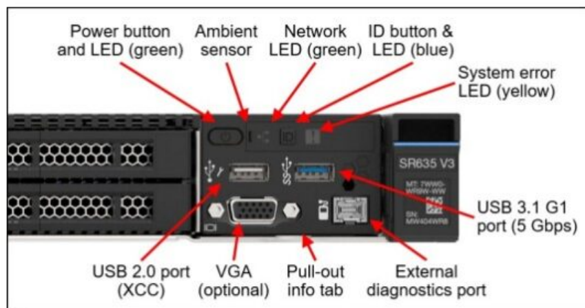
Figure 16. Front operator panel
