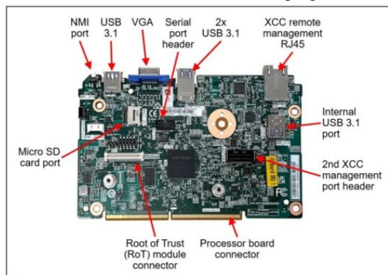
Figure 15. System I/O Board
