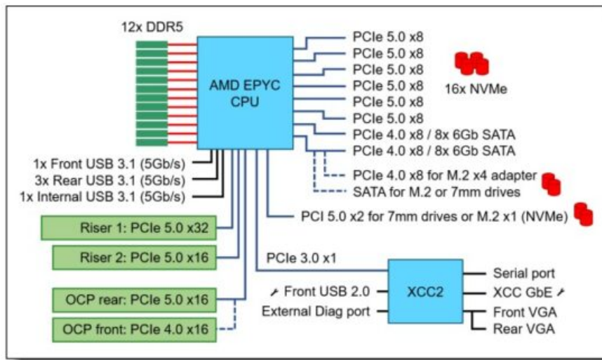
Figure 5. SR635 V3 system architectural block diagram
