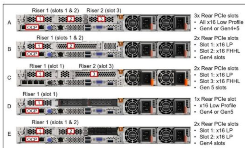
Figure 11. SR635 V3 slot configurations
