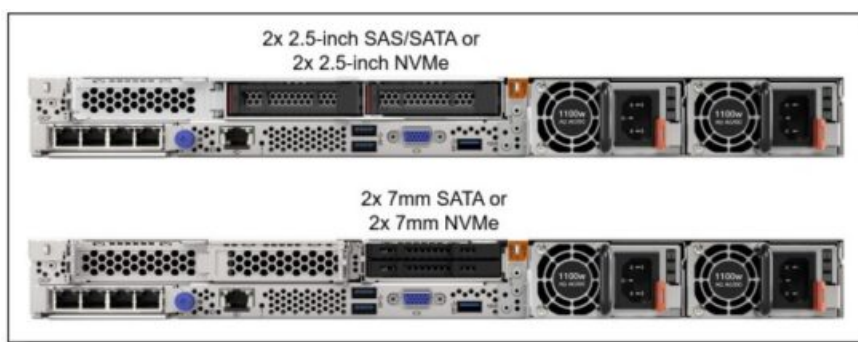
Figure 9. Rear drive bay configurations
