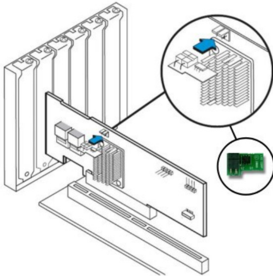
Figure 2. ServeRAID M1000 Series Advanced Feature Key
