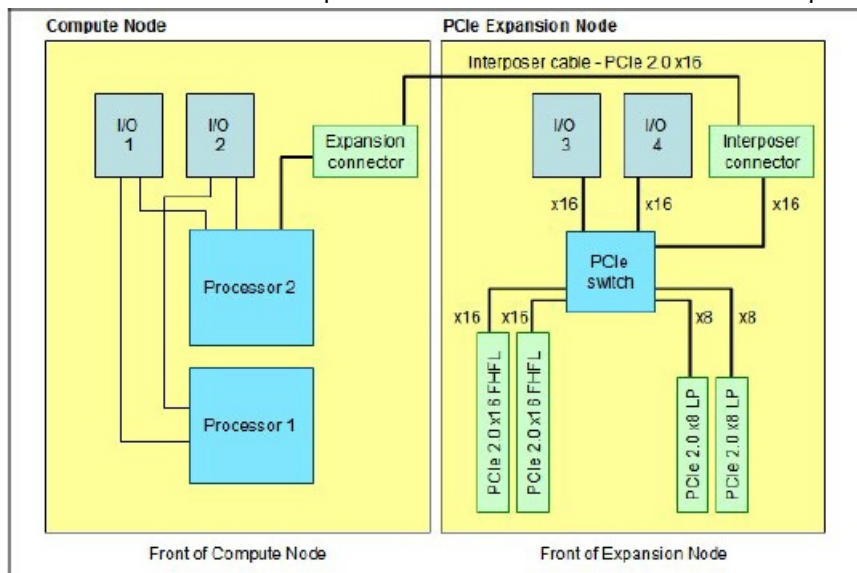
Figure 4. Architecture of the PCIe Expansion Node
