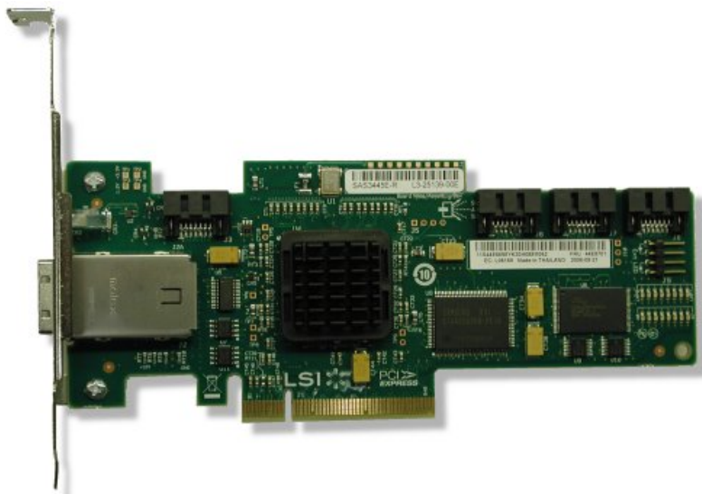
Figure 1. IBM 3Gb SAS HBA v2
