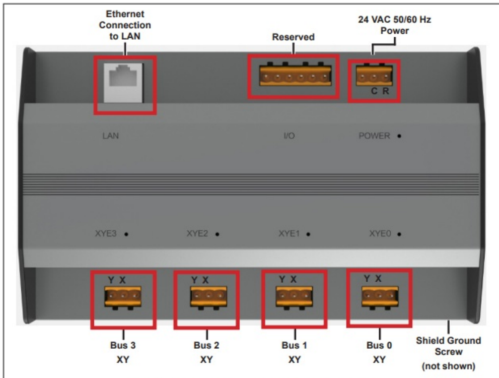
Figure 1. VRF BACnet Gateway Connection Points
