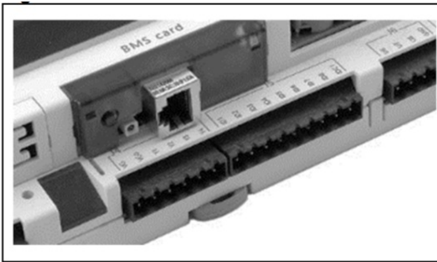
Figure 2.6 – LonWorks Card Installed
