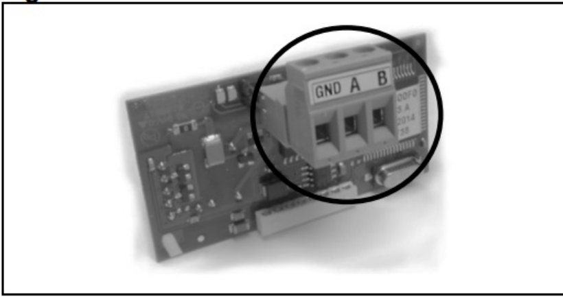
Figure 2.2 – LonWorks: Remove Connector
