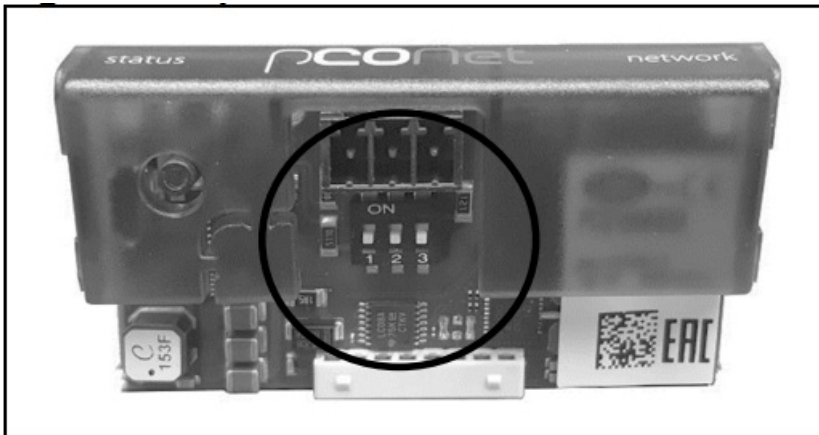
Figure 2.3 – pCONet: Set DIP Switches
