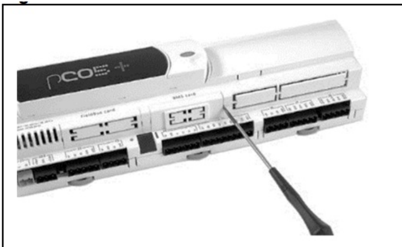
Figure 2.1 – Interface Card Location
