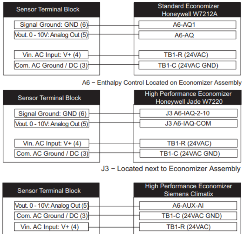
Figure 6. Field Wiring for KC/KG/KH, ZC/ZG/ZH and ELA units without Unit Controller
