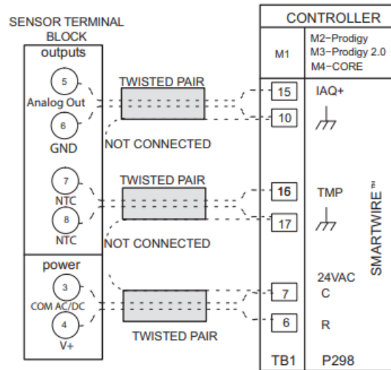
Figure 4. Field Wiring - 150' (46m) or Shorter Runs
