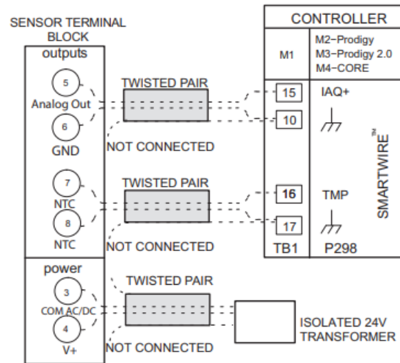
Figure 5. Field Wiring - 150' (46m) or Longer Runs
