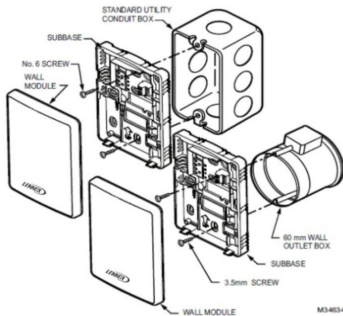
Figure 3. Installing Sub-Base on the Wall
