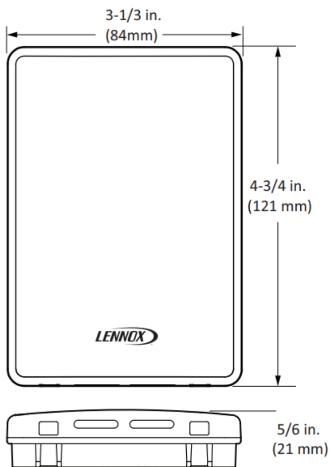
Figure 1. Carbon Dioxide Sensor Dimensions
