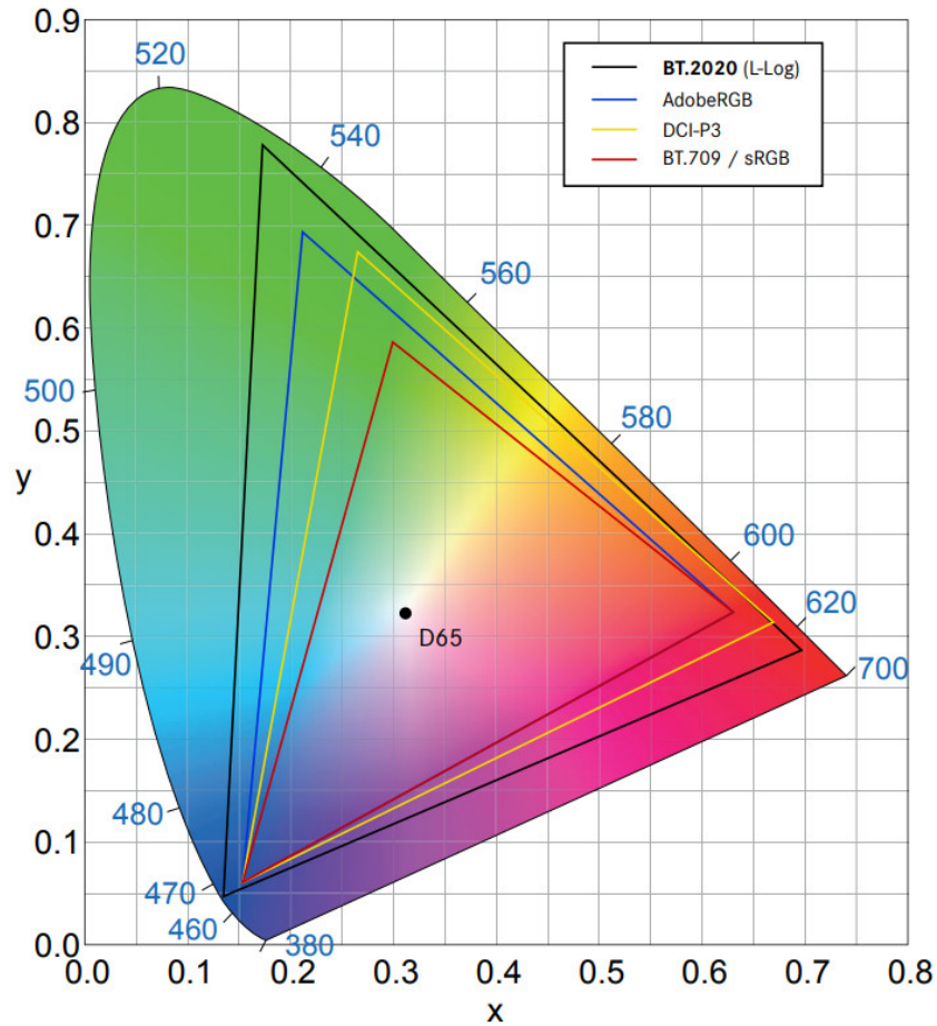
Figure 5: Comparison of color spaces.
