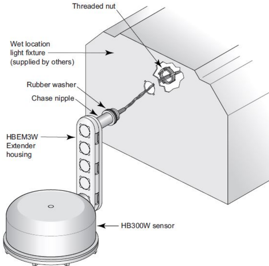
HB300W attached to a watertight light fixture using HBEM3W
