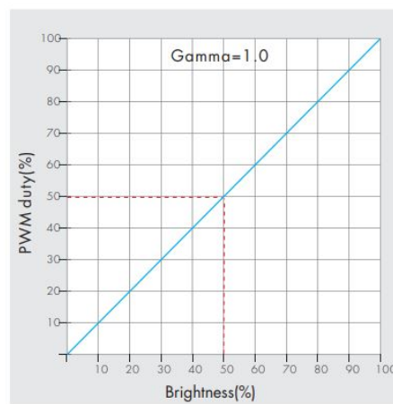
Dimming curve
