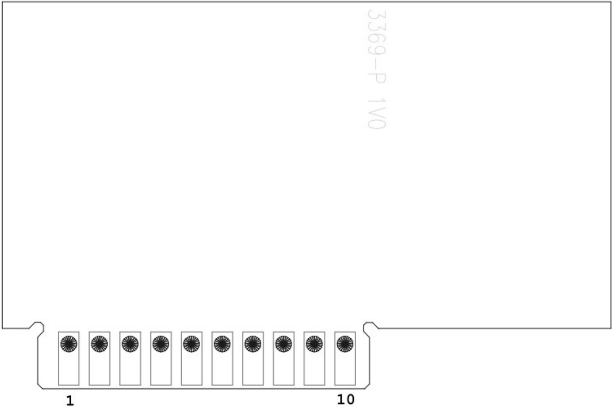
Fig 1 ML3369T-P pin sequence
