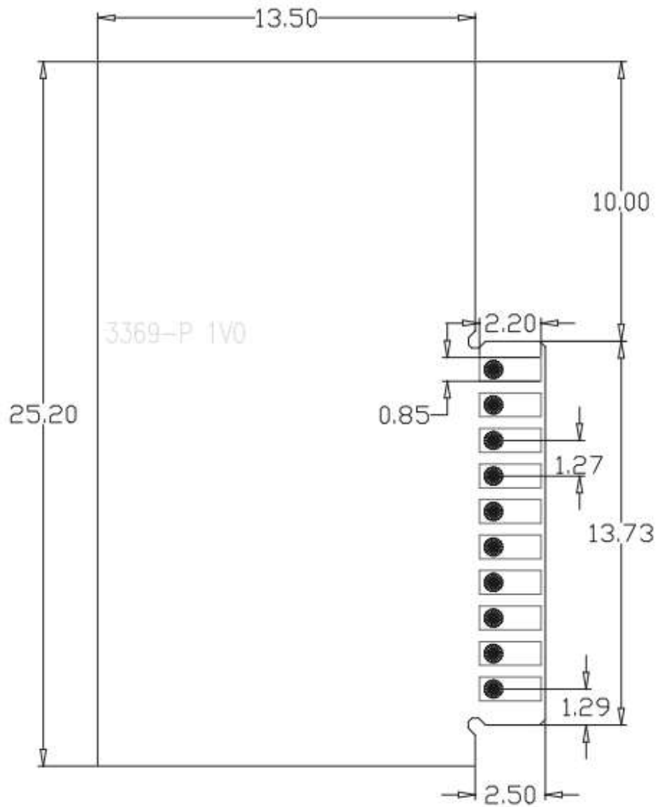
Fig 2 BL3369T-P Dimensions
