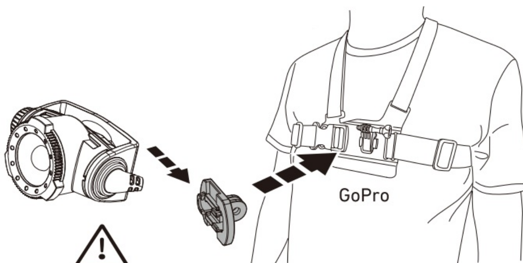
GoPro Mount (H7R Signature)
