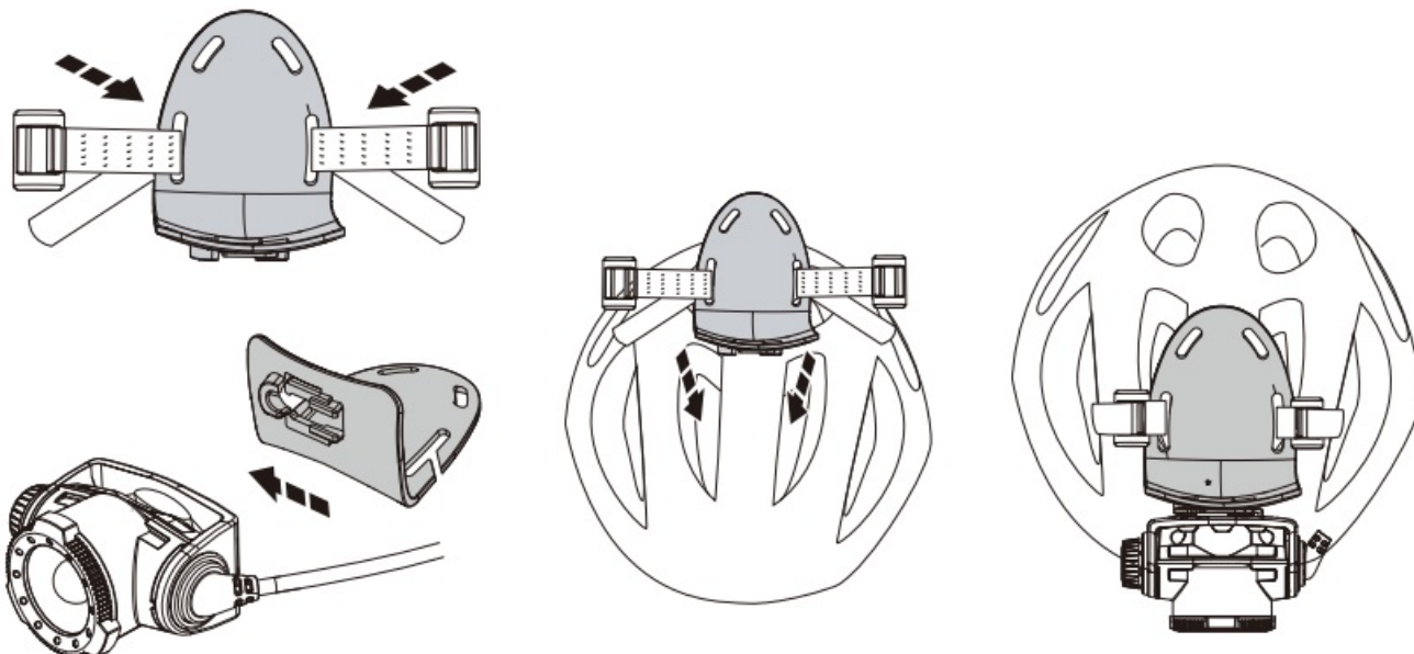
Helmet Fixing Clips (H7R Work & H7R Signature)
