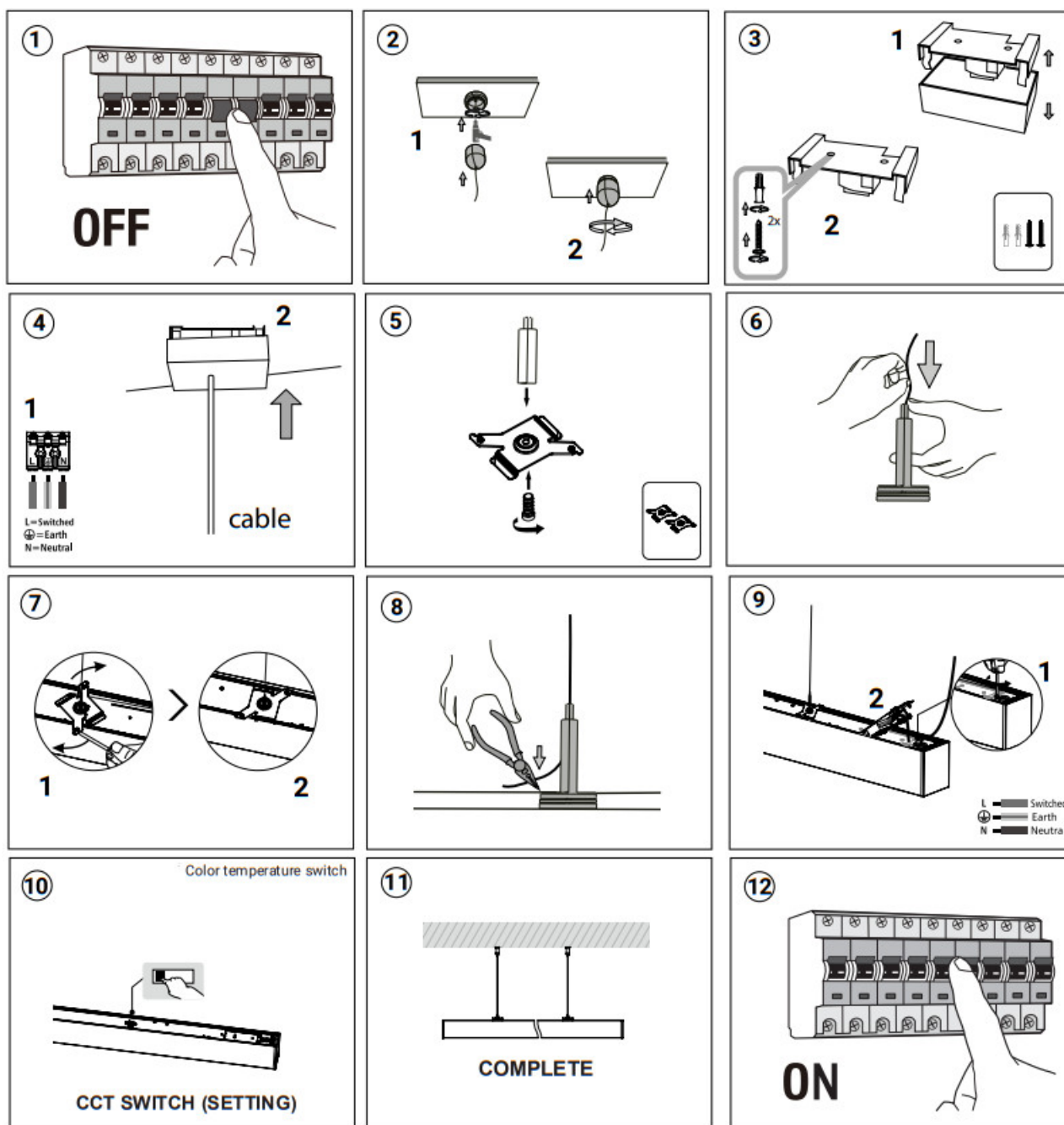
CONNECTION – DIMMABLE VERSION – OPTIONAL
