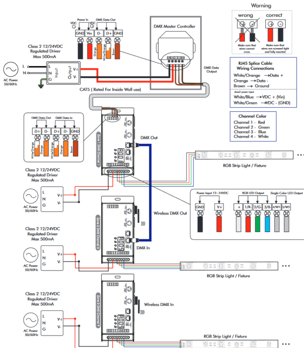
Method 2 : H-DMX2108A-5M-3 DMX Decoder
