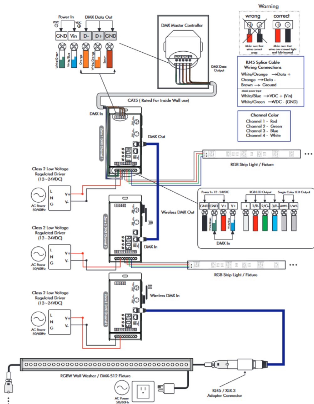
Method 1 : LT-840-6A DMX Decoder
