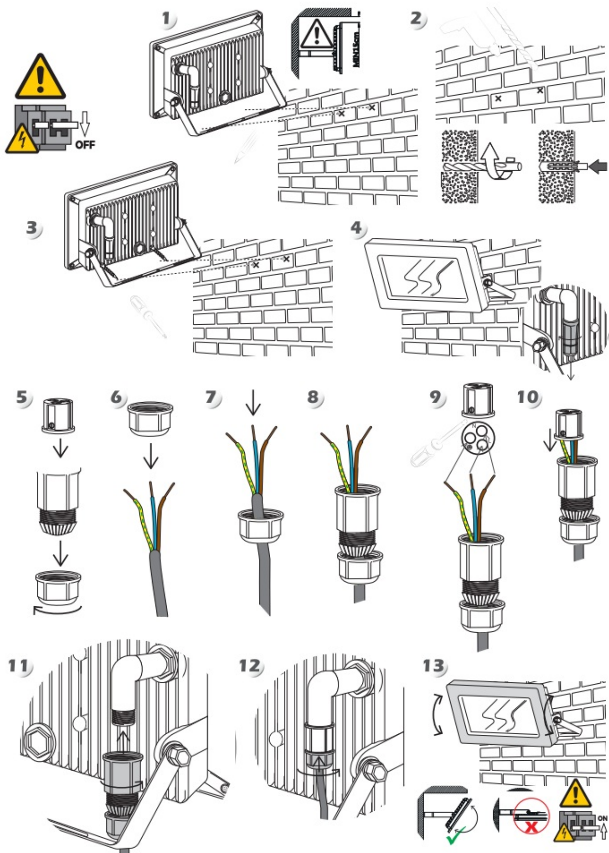
LED module replacement
