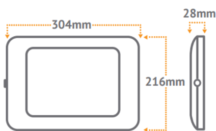
Enclosure 9" - 11"
