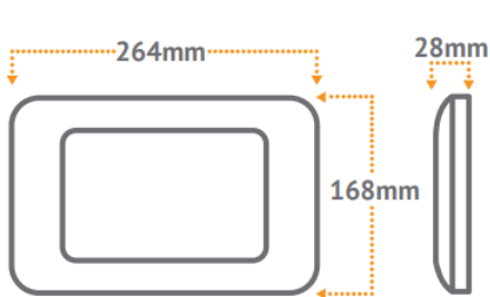
Enclosure 7"-9"
