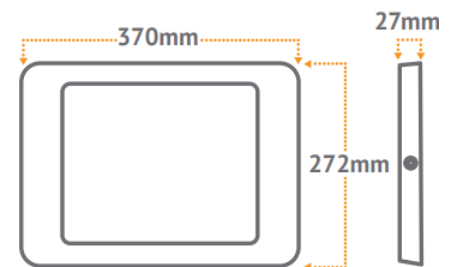
Enclosure 12.9
