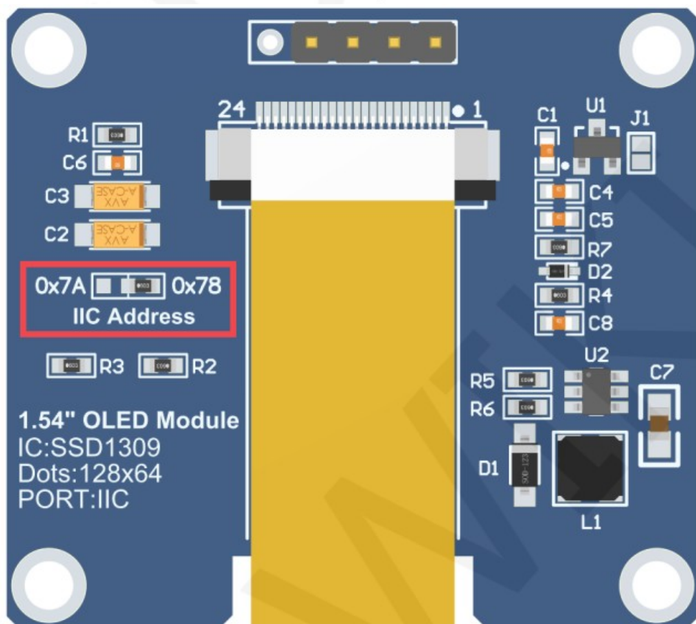
Picture 1. Module pin silk screen
